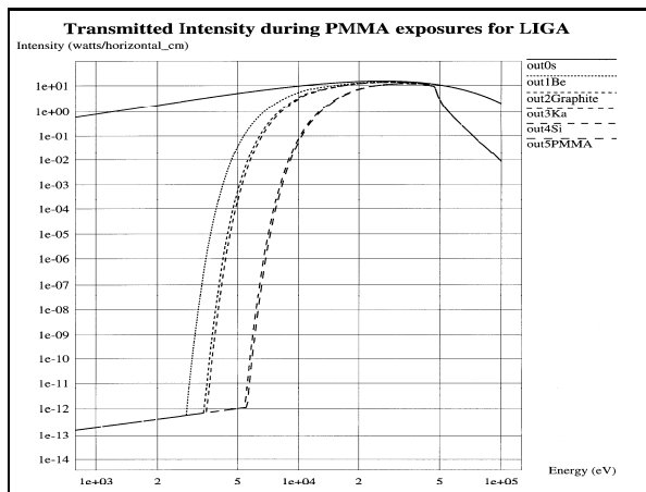
Figure 2: Transmitted x-ray intensity during PMMA exposures for DXRL at APS, energy vs. intensity.
