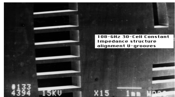
Figure 4: Scanning electron microscopy picture of the 108-GHz constant-impedance cavity structure.
