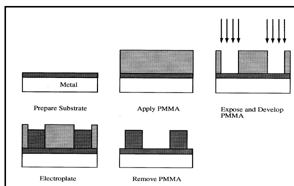
Figure 1: Simplified DXRL process.
