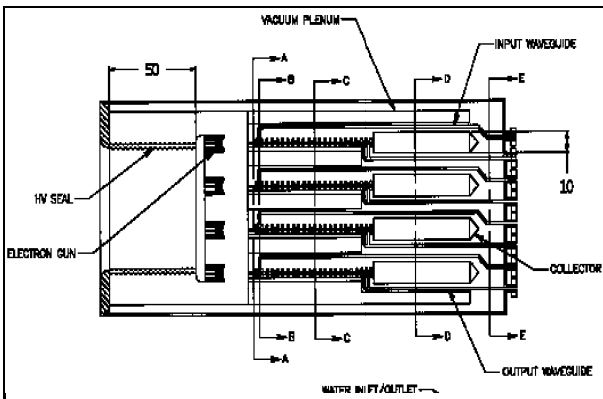
Figure 4: Four-klystron module layout.
