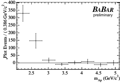
Figure 2: Efficiency corrected sPlot of m_{\bar{\Lambda}p} distribution for signal events.
