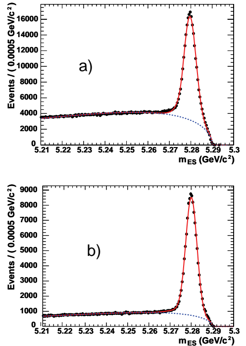
FIG. 1: m_{\text{ES}} spectra of reconstructed (a) B^+ and (b) B^0 candidates. The solid curve is the sum of the fitted signal and background whereas the dashed curve is the background component only.
