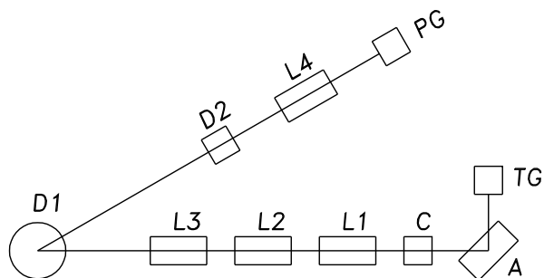
Figure 1: The layout of the SSRL injector and the gun test stand showing thermionic and photocathode gun (TG, PG), alpha magnet(A), chopper(C), linacs (L1 through L4), and dumps (D1, D2).
