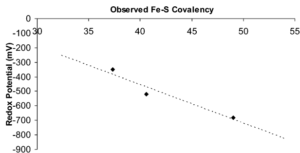
Figure 6. Plot of measured Fe–S covalency vs redox potential measured in CH 2 Cl 2 solution.
