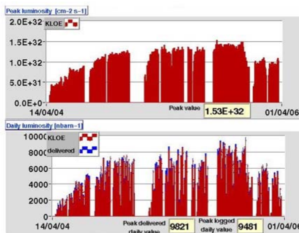
Figure 1: Last KLOE run peak and integrated luminosity.
