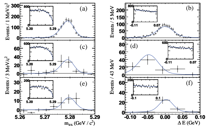
FIG. 1: Distributions of (left) m_{\text{ES}} and (right) \Delta E for signal (main plot) and background (inset) (a),(b) K_S^0\pi^+ , (c),(d) K_S^0K^+ , and (e),(f) K_S^0K_S^0 candidates (points with error bars) in data obtained with the weighting technique described in the text. The solid curves represent the assumed shapes used in the fits.
