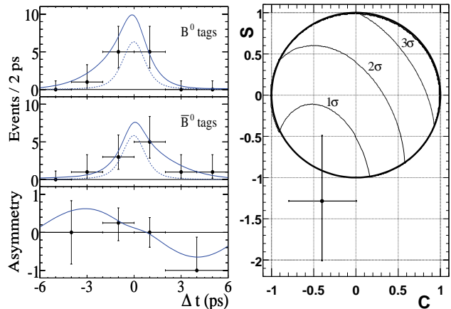
FIG. 2: Left: distributions of \Delta t for B^0 \rightarrow K_S^0K_S^0 decays in data tagged as B^0 (top) or \bar{B}^0 (middle), and the asymmetry (bottom). The data is enhanced in signal decays using requirements on probability ratios. The solid curve represents the PDF projection for the sum of signal and background, while the dotted curve shows the contribution from background only. Right: Likelihood contours in the S vs. C plane, where n\sigma corresponds to a change in -2\log\mathcal{L} of 2.3 for n = 1 , 6.2 for n = 2 , and 11.8 for n = 3 . The circle indicates the physically allowed region, while the point with error bars denotes the result of the fit to data.
