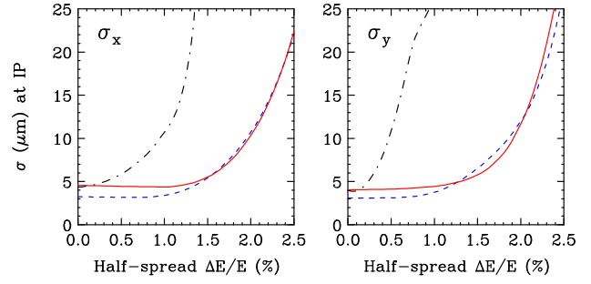
Figure 5: \sigma_{x,y} at IP versus half-width of a flat energy spread: a) with sextupoles and SR (solid line), b) with sextupoles and without SR (dashed line), and c) without sextupoles and with SR (dash-dot line).
