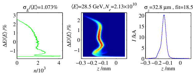
Figure 4: LiTrack longitudinal beam distribution at IP for the nominal case: \Delta E/E , phase space, bunch length.
