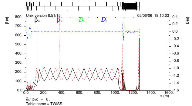
Figure 3: \beta functions and dispersion in SABER from the linac Sector-20 extraction point to the final focus IP.
