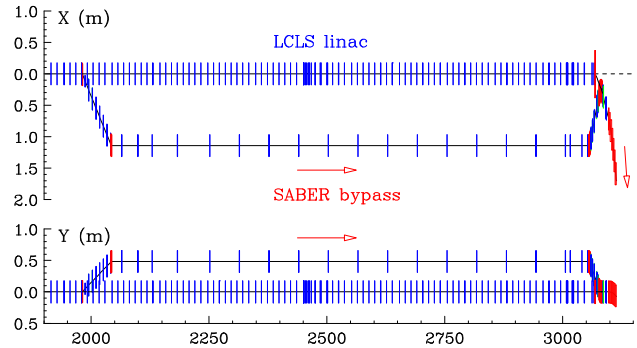
Figure 2: Geometrical layout of bypass magnets.
