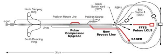
Figure 1: SABER at the SLAC accelerator facility.
