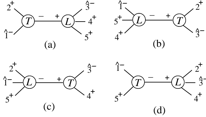
FIG. 4: Non-vanishing recursive diagrams for the amplitude A_{5;1}^{\mathcal{N}=0}(1^-, 2^+, 3^-, 4^+, 5^+) , using a [1, 3] shift, as given in eqs. (4.11)-(4.14).
