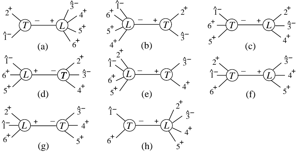
FIG. 6: Non-vanishing recursive diagrams for the amplitude A_{6;1}^{N=0}(1,3) , using a [1,3\rangle shift, as given in eq. (4.23).
