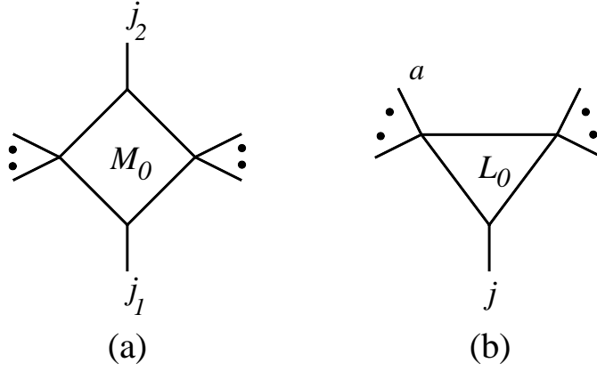
FIG. 11: Kinematic configuration of the box and triangle functions appearing in the completed-cut contribution given in eq. (A1).
