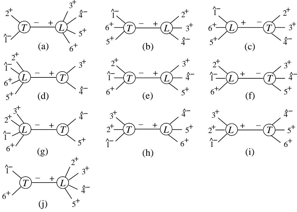
FIG. 8: Non-vanishing recursive diagrams for the amplitude A_{6;1}^{\mathcal{N}=0}(1,4) , using a [1,4\rangle shift, as given in eq. (4.25).
