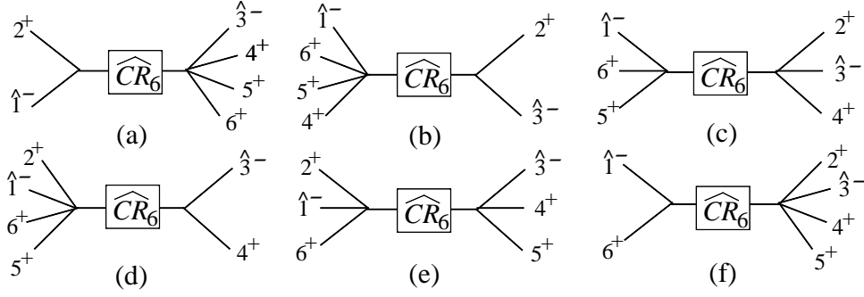
FIG. 7: Channels that can give overlap contributions to A_{6;1}^{N=0}(1,3) with a [1,3] shift, at the values of z given in eq. (4.24).
