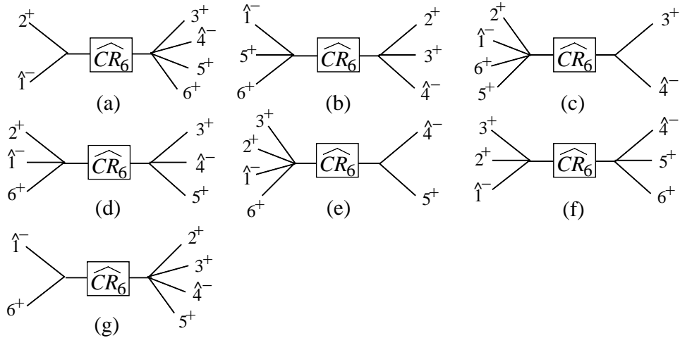
FIG. 9: Channels giving overlap contributions to A_{6;1}^{\mathcal{N}=0}(1,4) with a [1,4\rangle shift, at the values of z given in eq. (4.26).
