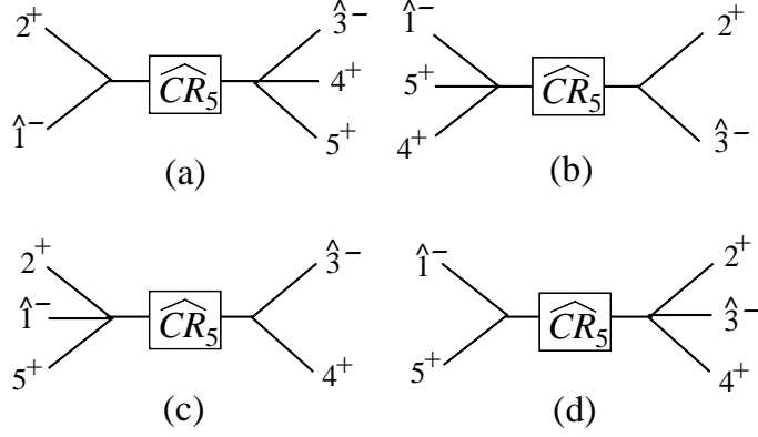
FIG. 5: Channels giving overlap contributions to A_{5;1}^{N=0}(1^-, 2^+, 3^-, 4^+, 5^+) with a [1, 3] shift, at the values of z given in eq. (4.15).
