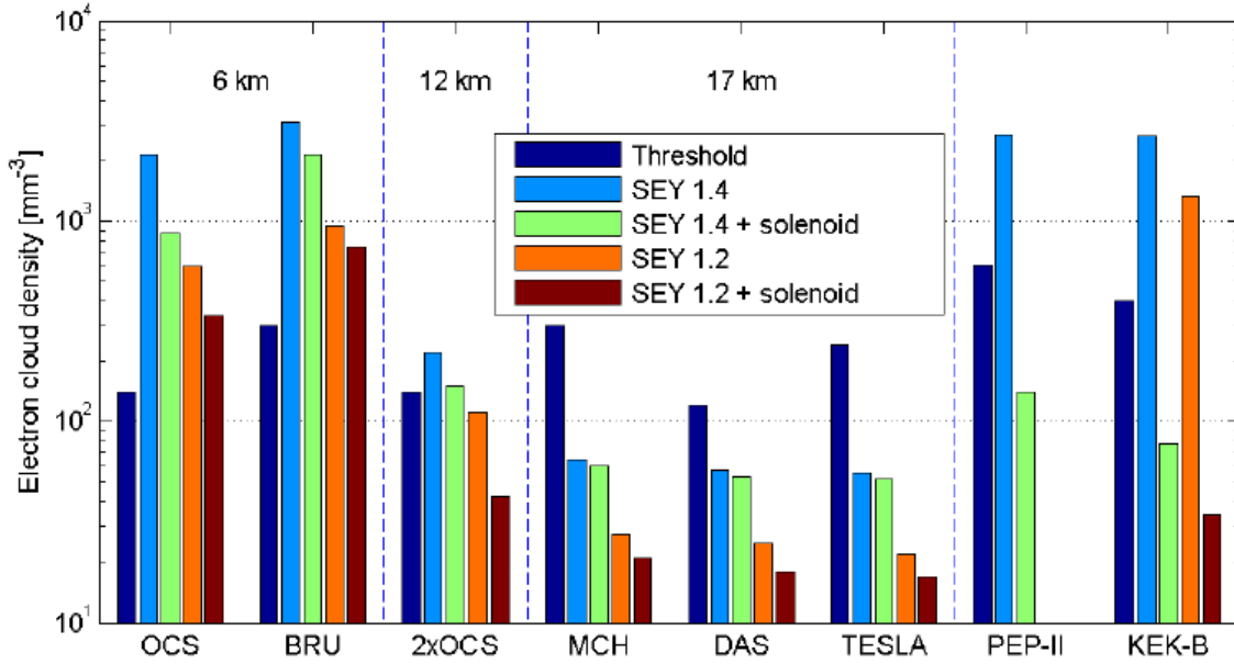
Figure 1: Instability thresholds and cloud densities for various SEY and solenoid combinations in the different damping ring configuration and the B factories. A wiggler vertical full of 18 mm is assumed in these simulations..
