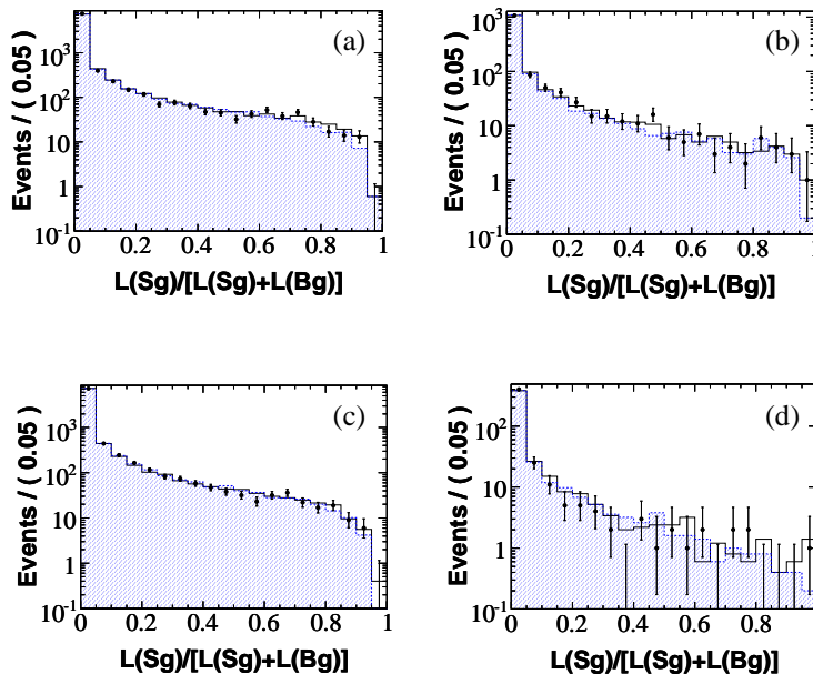
FIG. 2: The likelihood ratio L(\text{Sg})/[L(\text{Sg})+L(\text{Bg})] for the sub-decay modes of \eta'\eta'K : (a) \eta'\eta'\pi\eta'\rho\gamma K^+ , (b) \eta'\eta'\pi\pi\eta'\eta'\pi\pi K^+ , (c) \eta'\eta'\pi\pi\eta'\rho\gamma K_S^0 , (d) \eta'\eta'\pi\pi\eta'\eta'\pi\pi K_S^0 . The on-resonance data are shown as points with error bars; the sum of all simulated background samples is shown by the shaded (dashed-line) histograms; and the sum of these backgrounds plus the signal from the PDF model are given by the open (solid-line) histograms.
