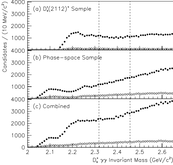
FIG. 28: The D_s^{*+}\gamma\gamma invariant mass distribution (solid points) for candidates in (a) the D_s^*(2112)^+ sample, (b) the non-resonant sample, and (c) either sample. The open points are the corresponding distributions for the D_s^{*+} sideband. The vertical dashed lines indicate the D_{s,J}^{*+}(2317)^+ and D_{s,J}^{*+}(2460)^+ meson masses.
