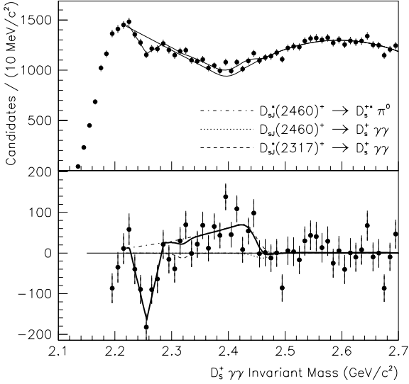
FIG. 30: The D_s^+ \gamma\gamma invariant mass distribution for the D_s^*(2112)^+ sample is shown on top. The thick curve is the result of the likelihood fit. The mass distribution after subtracting the portion assigned by the fit to combinatorial background is shown on bottom.
