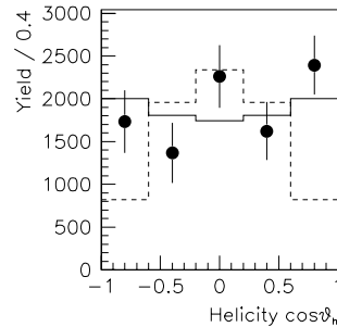
FIG. 24: Efficiency-corrected yields in five \cos \vartheta_h bins for the decay D_{sJ}(2460)^+ \rightarrow D_s^*(2112)^+\pi^0 . The solid histogram is the result of a fit to the function described in the text. The dashed histogram is a similar fit with the a_2 parameter fixed to zero.
