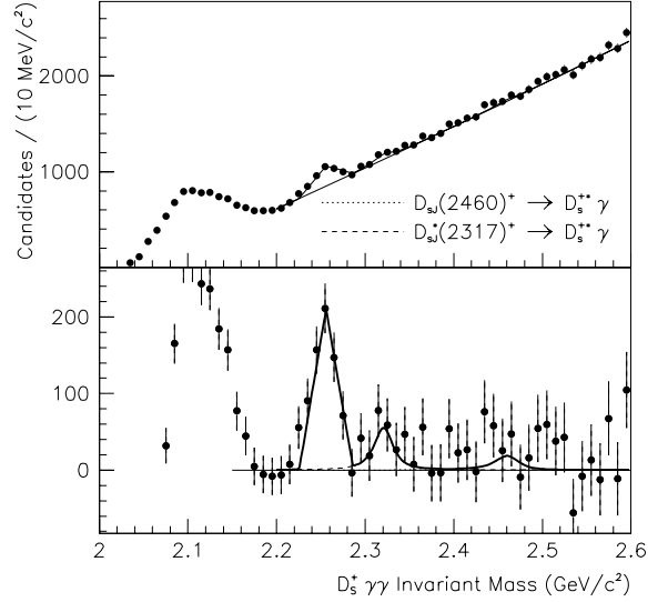
FIG. 31: The D_s^+ \gamma\gamma invariant mass distribution for the non-resonant sample is shown on top. The thick curve is the result of the likelihood fit. The mass distribution after subtracting the portion assigned by the fit to combinatorial background is shown on bottom.
