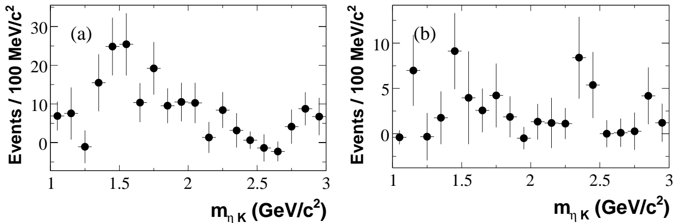
FIG. 2: Plot of \eta K invariant mass for signal using the weighting technique described in the text for the combined sub-decay modes: (a) charged modes, (b) neutral modes.
