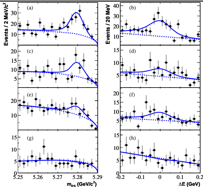
FIG. 1: The B candidate m_{ES} and \Delta E projections for \eta K^+ \gamma (a, b), \eta K^0 \gamma (c, d), \eta' K^+ \gamma (e, f) and \eta' K^0 \gamma (g, h). Points with error bars represent the data, the solid line the full fit function, and the dashed line its background component.
