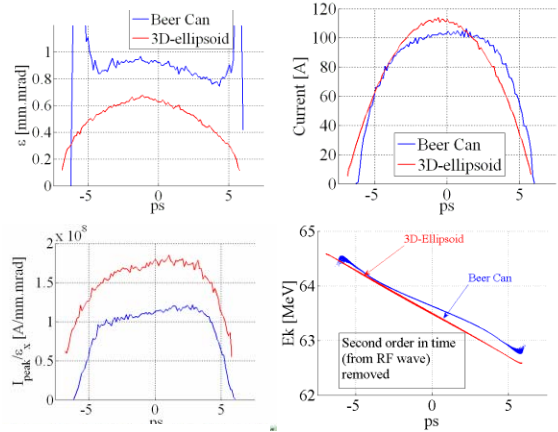
Figure 4: Blue and Red are for “Beer Can” (nominal LCLS tuning) and “3D-Ellipsoid” (LCLS case) (a) Slice emittance at end beamline – (b) Peak current – (c) Ratio of peak current over emittance – (d) Longitudinal Phase Space after removal of 2 nd order term in polynomial fit.
