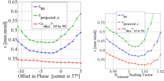
Figure 2: Sensitivity to Injection Phase (a) and to Solenoid field variation (b) (solenoid reference is 2.7kG).
