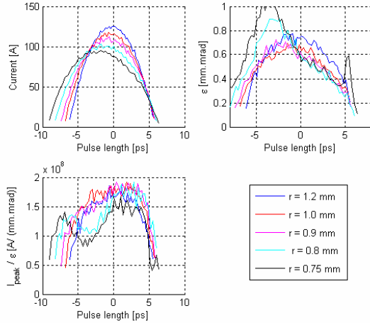
Figure 5: Beam characteristics at the end of the beamline as a function of the r parameter of equation (1)- (a) Peak Current- (b) Slice Emittance - (c) Ratio Peak Current over Emittance.
