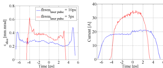
Figure 1: Slice emittance and peak current for 0.2nC Two cases correspond to fwhm laser pulse of 5 and 10ps.
