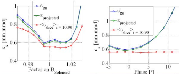
Figure 6: Emittance as a function of Solenoid field (a) with the field normalized to 2.7kG (a) and of Injection Phase (b) the reference phase is 27^\circ .
