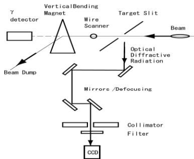
Figure 1: A Schematic Diagram of the Experiment.
