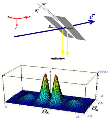
Figure 2: A schematic diagram of a disphased target slit to measure the vertical beam size and the ODR photon yield in the far field zone.
