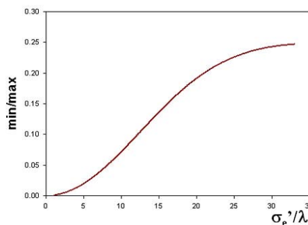
Figure 5: min/max ODR photon yield ratio as a function of the transverse beam size with the curved disphased target.
