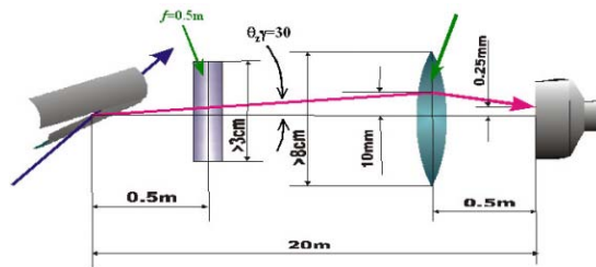
Figure 4: Lens Optics system for a disphased conductive slit target with curved surface.
