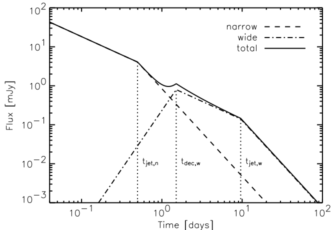
FIG. 3.— R-band lightcurve from a two-component model with parameters appropriate to GRB 030329 ( D_L = 0.8 Gpc): \eta_w = 8.7 , \eta_n = 200 , E_w = 1.1 \times 10^{51} ergs, E_n = 2.2 \times 10^{50} ergs, \theta_{j,w} = 0.26 , \theta_{j,n} = 0.093 , n_0 = 0.33 \text{ cm}^{-3} , \epsilon_e = 0.01 , \epsilon_B = 0.005 , and p = 2.25 .
