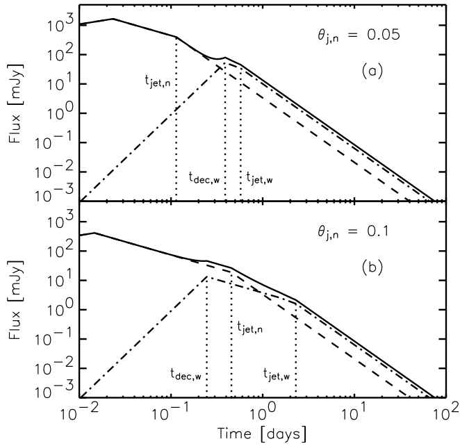
FIG. 2.— Similar to Fig. 1, except that E_w = 2 E_n and \theta_{j,w} = 2 \theta_{j,n} . The top and bottom panels correspond to \theta_{j,n} = 0.05 and 0.1, respectively. The other parameters are the same as in Fig. 1.
