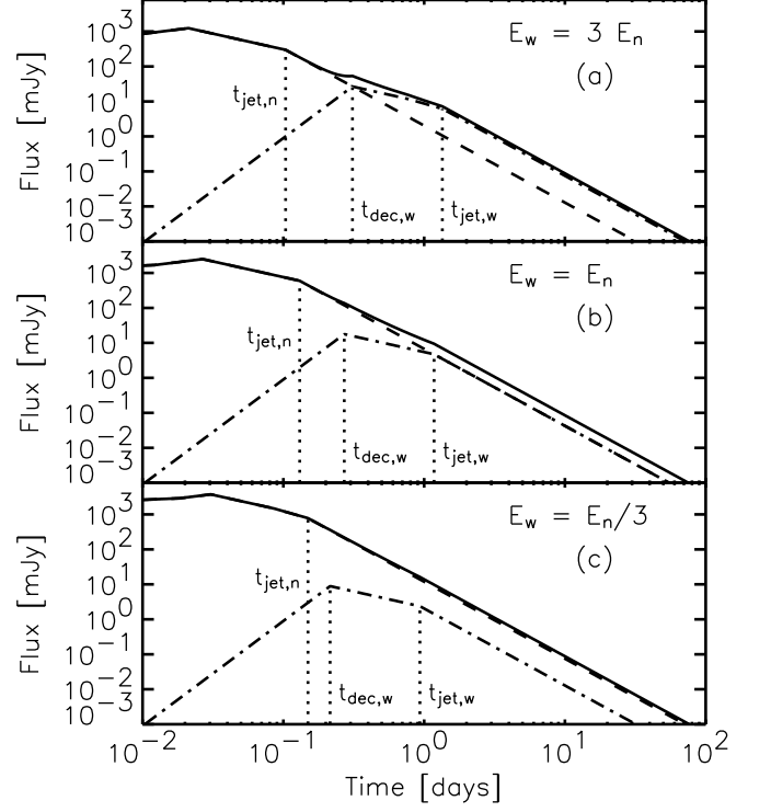
FIG. 1.— R-band afterglow lightcurve from a two-component jet. The contribution of the narrow component, wide component, and their sum is represented by the dashed, dash-dotted, and solid curves, respectively. The total outflow energy is assumed to be constant, E_w + E_n = 10^{51} ergs. From top to bottom, the 3 panels correspond to E_w/E_n = 3, 1, and 1/3 , respectively. The other parameters are the same for all panels: \eta_w = 15 , \theta_{j,w} = 0.15 , \theta_{j,n} = 0.05 , n_0 = 1 , \epsilon_e = 0.1 , \epsilon_B = 0.01 , p = 2.2 , and \tilde{D}_{L,28} = 1 .
