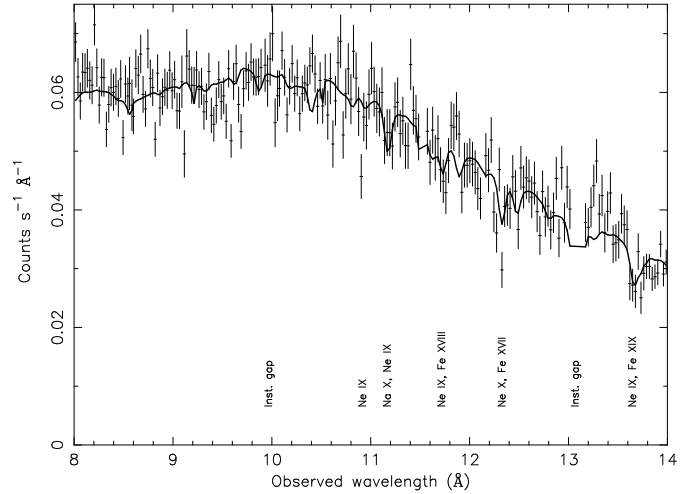
Fig. 8. Detail of the RGS spectrum between 8 and 14 Å. The solid line through the data points is our best fit model as described in the text. RGS 1 and 2 are added for clarity in this and the next two spectra.
