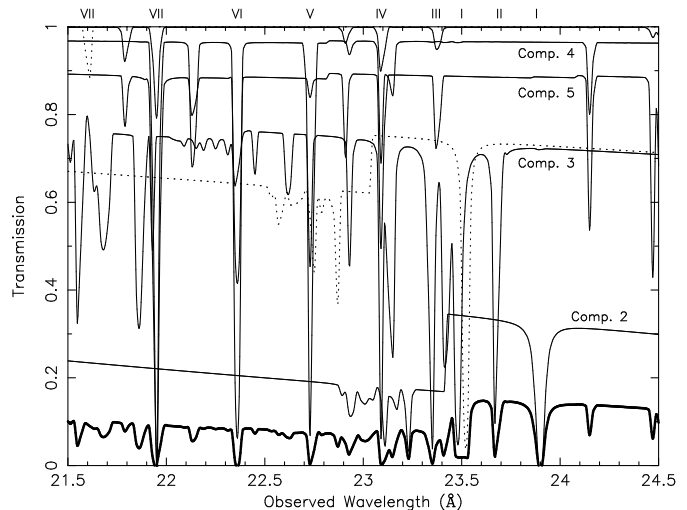
Fig. 13. Part of the spectrum detailing the transmission for the seven different absorption components. The thick line indicates the best fit spectral model, i. e. with all seven absorption models applied. The dotted line at the top with only an O VII absorption line is component 7, the other dotted line is component 1, or Galactic absorption. The solid line on the top represent component 6, the other components are labeled in the plot. In roman numerals the ionization state of oxygen is indicated, from neutral oxygen (I) to O VII (VII).
