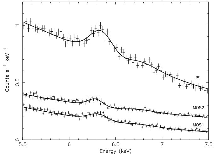
Fig. 5. Detail of the pn, MOS 1 and MOS 2 spectra showing the Fe K\alpha and Fe XXVI Ly \alpha emission lines. The model through the data is given in Table 3. The MOS 2 data were shifted by adding 0.006 counts s -1 for clarity.
