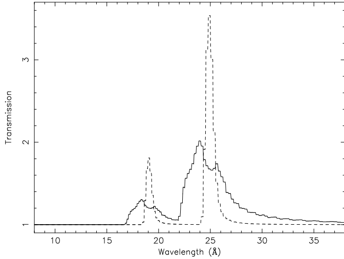
Fig. 7. Models for the two broadened emission features detected in the RGS spectrum (see Sect 5.4) and the two emission features detected in the pn spectrum. The thin solid line represents the best fit for the relativistically broadened lines detected in the RGS spectra, with q = 1.9 and i = 80.9 (see Table 7). The dashed line represents the model for the emission features adopting the parameters found for the relativistically broadened Fe K\alpha and Fe XXVI emission lines: emissivity slope q = 1 and i = 12^\circ , consistent with the values obtained by McKernan & Yaqoob (2004). Note that this profile is very similar to a Gaussian profile.
