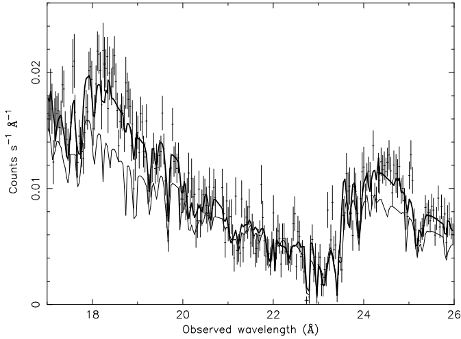
Fig. 14. The best fit model with the disklines fit (thick line) versus the model without these excesses fit (thin line).
