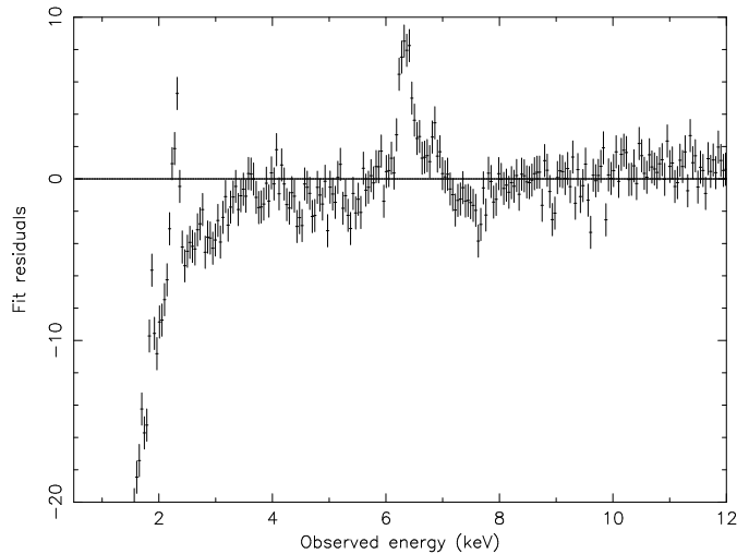
Fig. 6. A power-law plus Galactic absorption fit to the pn spectrum, rebinned by a factor of 9. Note the Fe K\alpha and Fe XXVI Ly \alpha emission lines, as well as the absorption at lower energies. The feature at 2 keV is an artifact of the absorption spectrum and the soft excess. Note that the reflection component has at most a 1 \sigma significance.
