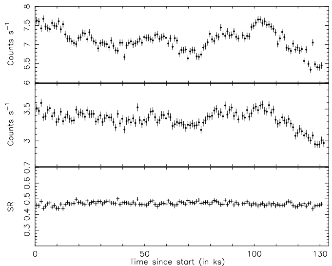
Fig. 2. Lightcurves for the pn instrument. Top: the hard band between 2 – 10 keV; middle: the soft band between 0.4 – 1 keV. Bottom: the softness ratio: the 0.4 – 1 keV count rate divided by the 2 – 10 keV count rate. All the data were binned in 1000 s bins.
