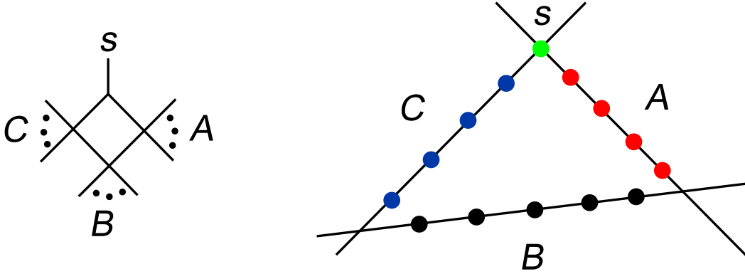
FIG. 8: The twistor-space configuration for the three-mass-box coefficients c^{3m} given in eq. (15) is depicted on the right. The corresponding three-mass integral is shown on the left. All points lie in a plane.
