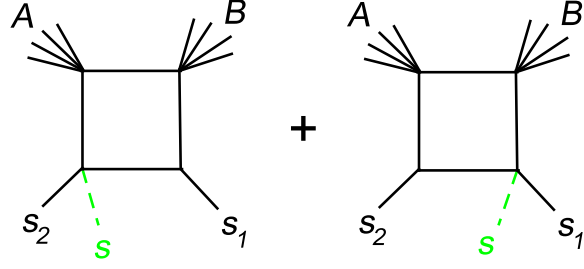
FIG. 6: The three-mass box integrals that may be used to verify all hard two-mass coefficients. Leg s becomes soft.
