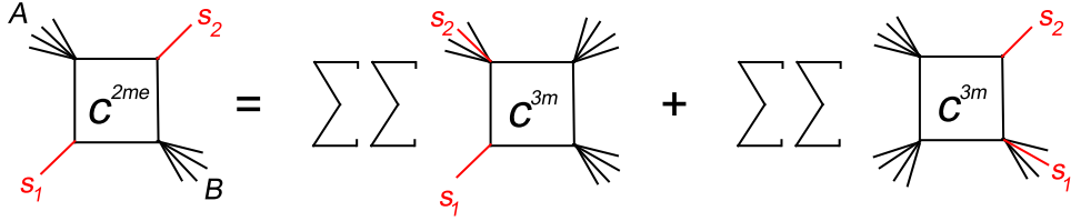
FIG. 4: Schematic depiction of the easy two-mass box coefficients, expressed as a double sum over three-mass box coefficients.
