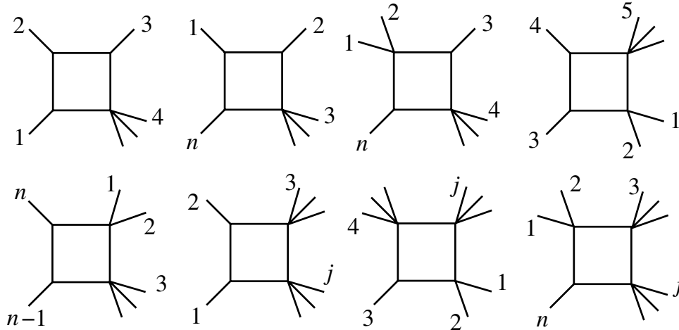
FIG. 7: The boxes whose coefficients combine to give one of the new representations of any one-loop n -point tree amplitude. These boxes are the ones with infrared singularities of the form \ln(-s_{12})/\epsilon .
