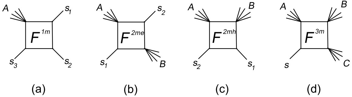
FIG. 3: The box integral functions labeled by the clusters of masses.
