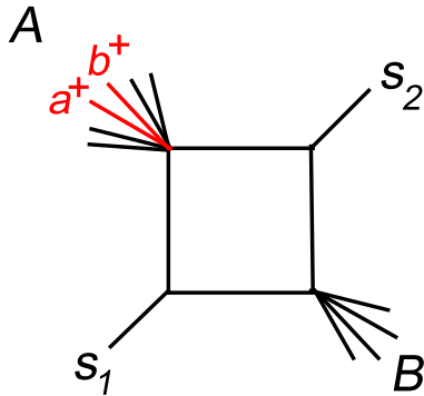
FIG. 5: An easy two-mass box where positive helicity legs a and b are buried inside a cluster.
