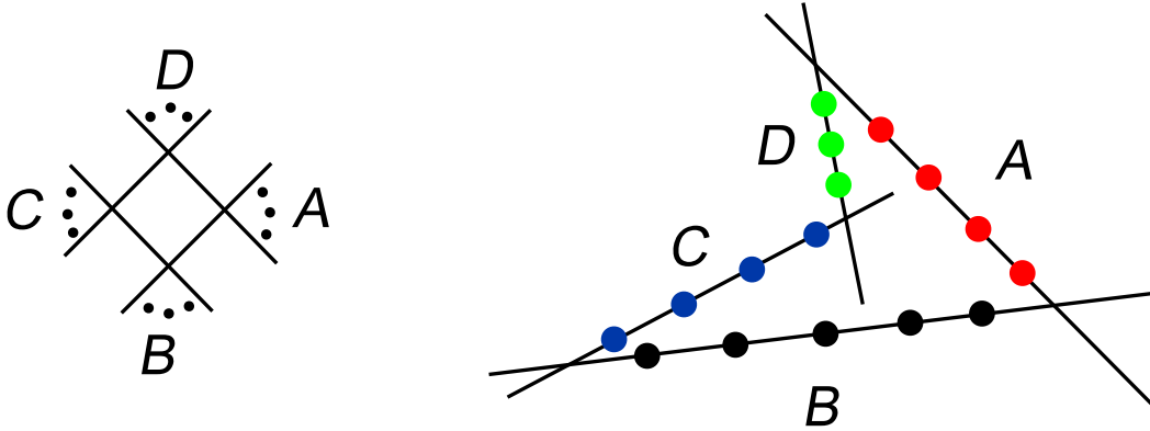
FIG. 9: The twistor-space configuration for the four-mass-box coefficient of an N^2 MHV amplitude is depicted on the right. The corresponding four-mass integral is shown on the left. The points need not lie in a plane, but lie in the intersection of two planes.
