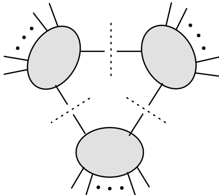
FIG. 2: A generalized triple cut. The three propagators cut by the dashed lines are required to be ‘open’.
