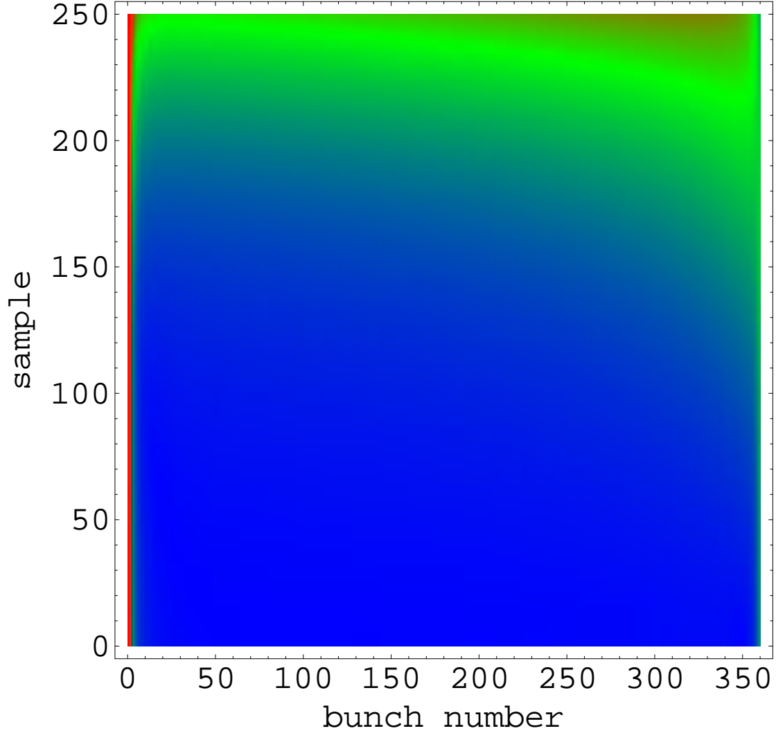
FIG. 5: Amplitude growth due to RW instability. All 360 modes are taken into account.
