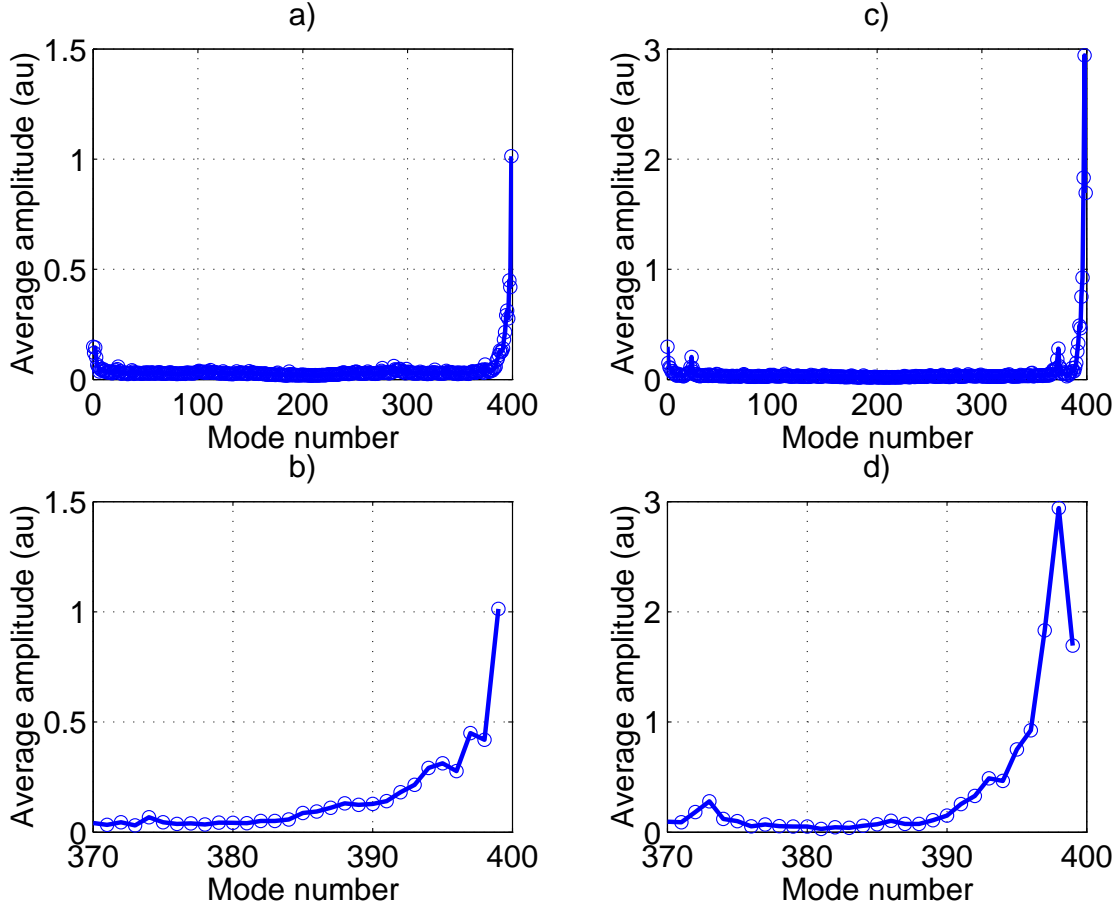
FIG. 2: Average modal amplitudes vs. mode number for the growth transient parts of two grow/damp experiments at BESSY-II. a) 320 bunches in the ring with an 80 bucket (20%) gap; b) Plot a) zoomed in; c) 400 bunches, no ion clearing gap; d) Plot c) zoomed in.
