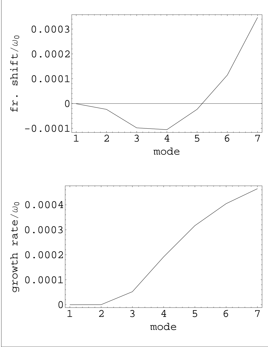
FIG. 14: Dimensionless coherent frequency \mu/\omega_0 of the beam-ion instability in the linear approximation.
