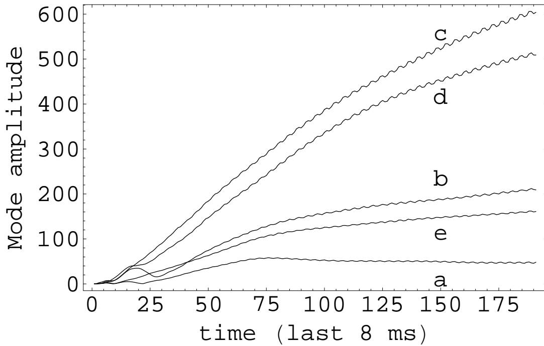
FIG. 11: Time variation of the strongest modes. 320 bunches in the ring.
