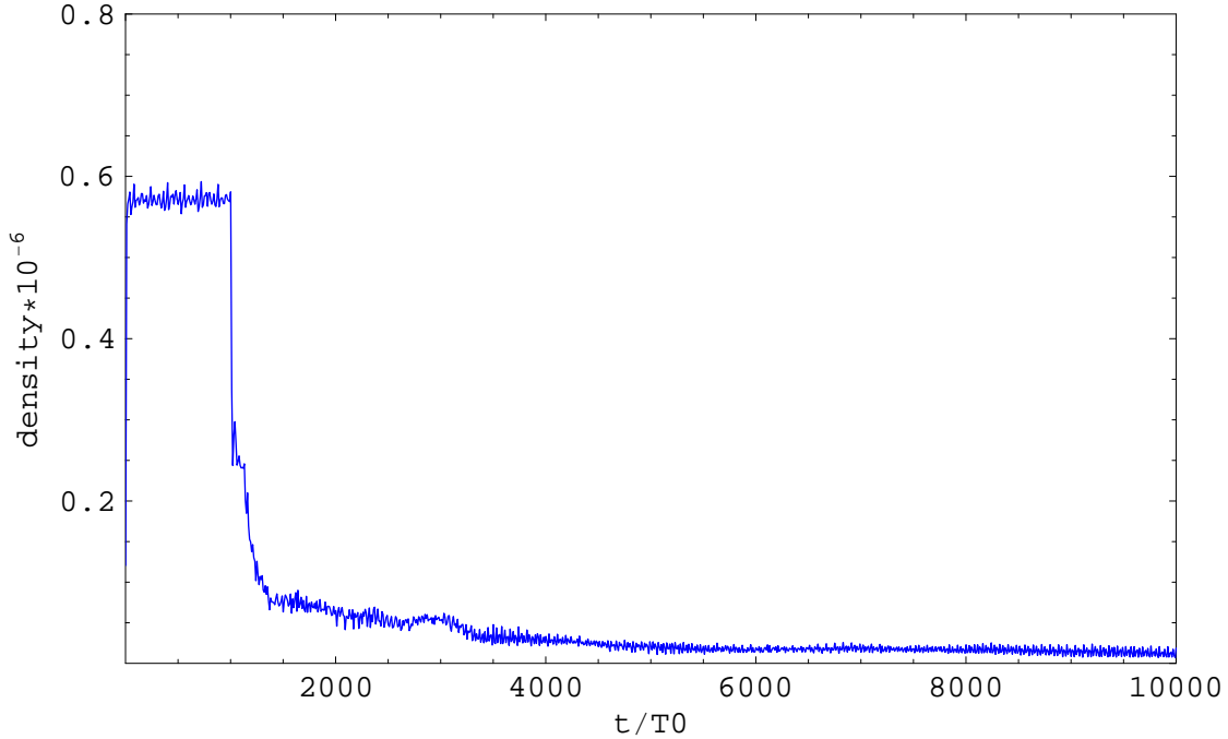
FIG. 13: Variation of the ion density with time for the train of 320 bunches. The density grows and saturates while the beam is kept stable for the first 1000 turns and then drops with the growth of the beam amplitude.
