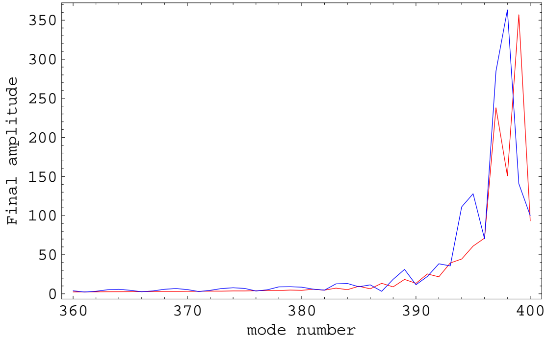
FIG. 10: Amplitude of CB modes |C_m| vs mode number taken at the end of tracking ( t = 16 ms) for the train n_b = 320 (blue) and n_b = 400 (red) bunches.
