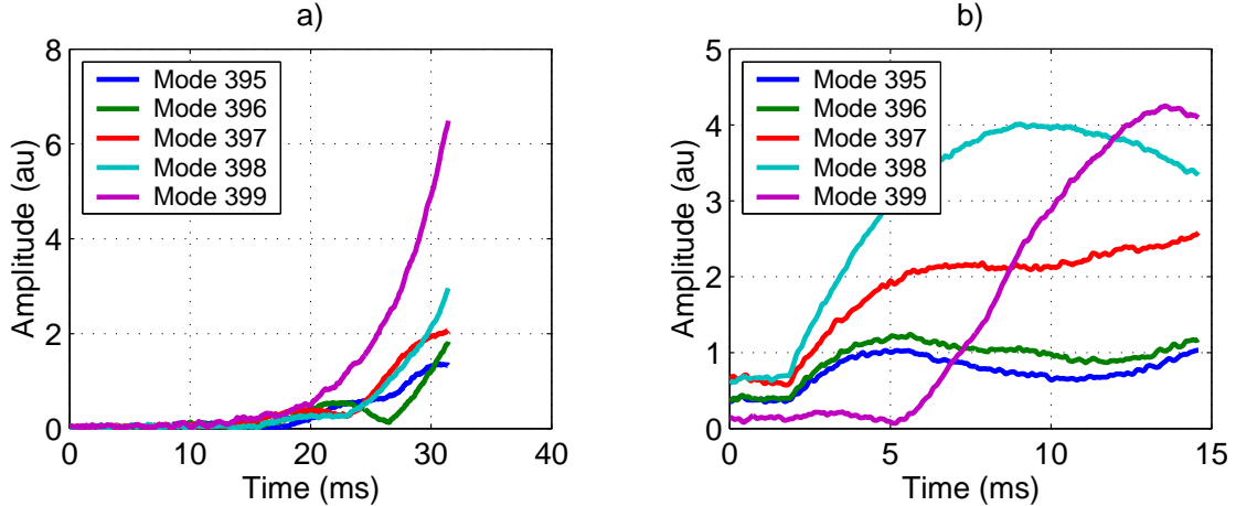
FIG. 3: Variation of the amplitude of several CB modes vs. time for two grow/damp experiments at BESSY-II. a) 320 bunches in the ring, 20% gap; b) 400 bunches, no ion clearing gap.
