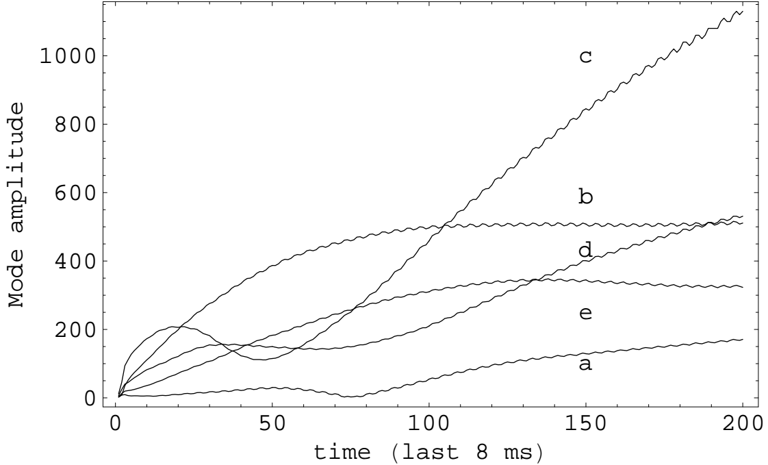
FIG. 12: The same as in Fig. 11 for the train of 400 bunches.
