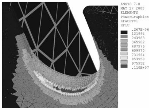
Figure 2 Localized heating of the RF coupling port on the full cell of the gun. The heat flux (watts/m 2 ) is shown for the gun operating at 140 MV/m and 120 Hz. The total dissipated power is 3676 watts.[8]
