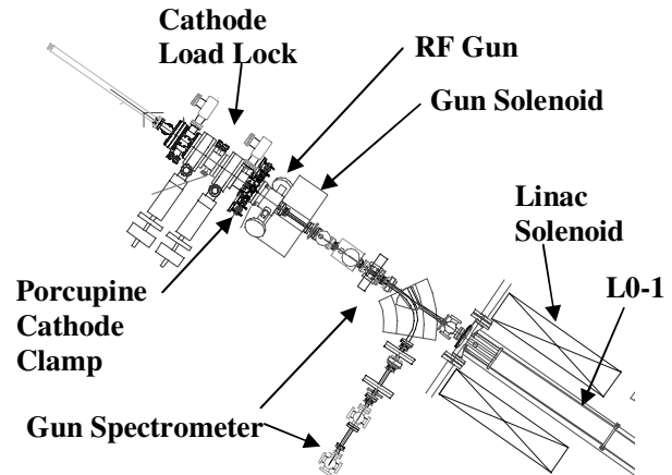
Figure 3 Low energy region of the injector.
