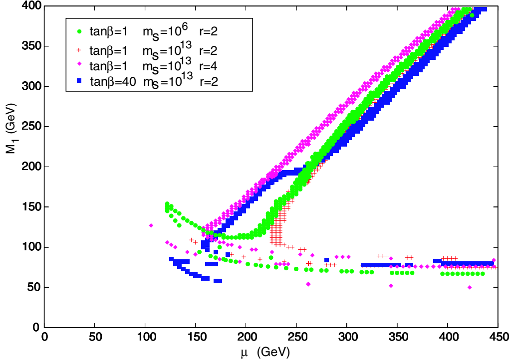
Figure 1: Points in the \mu - M_1 plane that satisfy the relic abundance constraint from WMAP. The region at low M_1 extending to large \mu is the Higgs resonance region; the dark matter can be very nearly bino in this region. The diagonal line represents a mixed bino-higgsino dark matter region. The allowed region is shown for various values of \tan\beta , scalar masses, m_S , and r \equiv M_2/M_1 . The top quark mass is set to 178 GeV.
