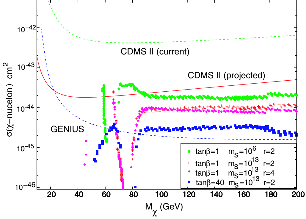
Figure 2: The spin-independent LSP-nucleon scattering cross-section for point agreeing with the WMAP relic density constraint. Curves are plotted for various values of m_S (the scale of the scalar masses), \tan\beta (set at m_S ), and r \equiv M_2/M_1 . The flat regions for m_\chi \gtrsim 80 GeV correspond to mixed bino-higgsino dark matter. The sharp decrease at lower masses is due to resonant annihilation through the Higgs boson and Z -boson poles. Also shown are the current bound from the results of the Cryogenic Dark Matter Search (CDMS) at Soudan [16], the projected bounds from this experiment [17], and projected bounds from a representative next generation dark matter experiment, GENIUS [18]
