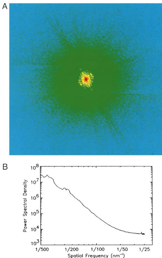
Fig. 1. (A) A diffraction pattern from E. coli bacteria displayed in a logarithmic scale. (B) The power spectral density of the diffraction pattern, which indicates the resolution extends to 30 nm.
