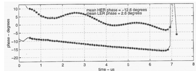
Figure 1. The variation of the bunch RF phase along the bunch train for the LER top and HER bottom. Note the three degrees relative variation in the LER.
