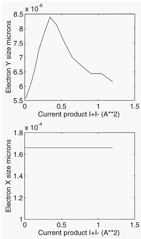
Figure 5. Measured HER electron beam sizes as a function of the product of the beam currents.
