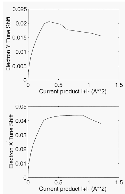
Figure 6. Derived beam-beam tune shift parameters versus current for HER electron.
