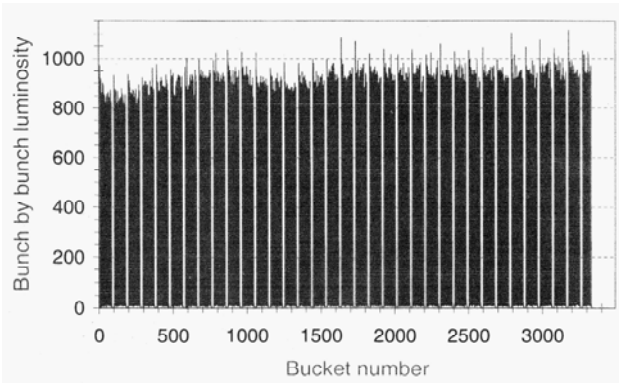
Figure 2. The measured luminosity in each bunch along the bunch train. Note that the luminosity dips where the LER RF phase has maxima.
