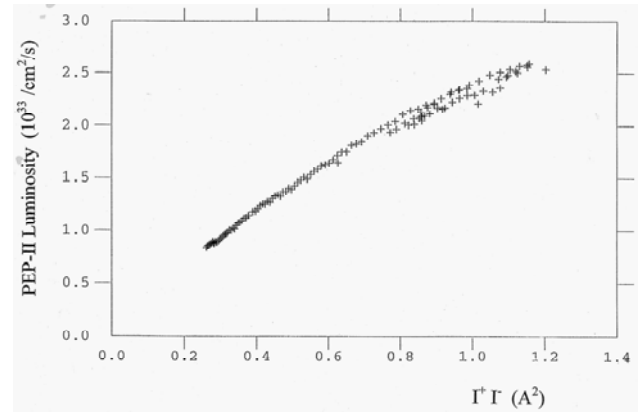
Figure 4. PEP-II luminosity versus the product of the beam currents. Note that the luminosity deviates from an ideal square law due to the enlargement of the beam sizes.
