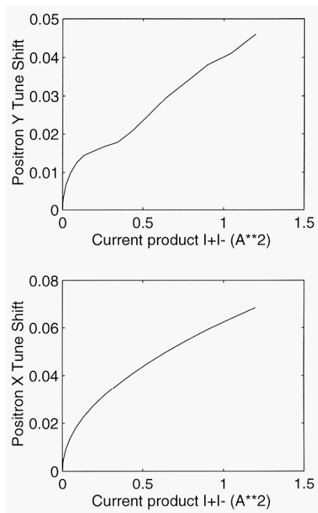
Figure 8. Derived beam-beam tune shift parameters versus current for LER positrons.
