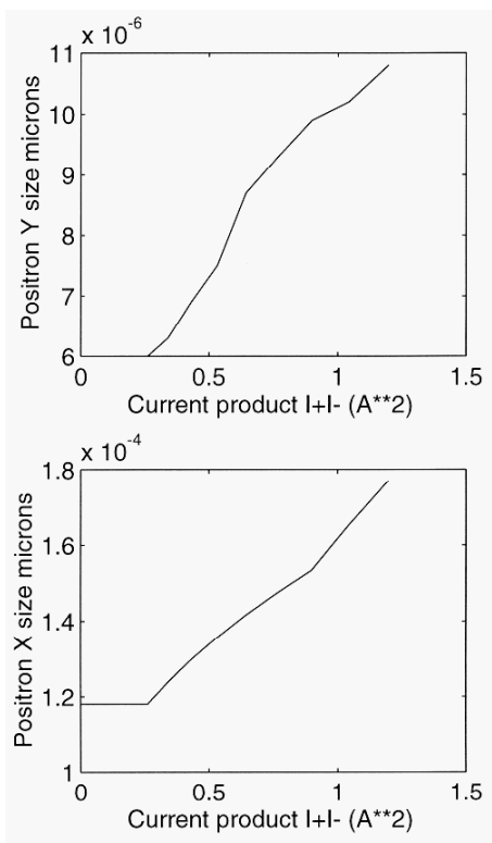
Figure 7. Measured LER positron beam sizes as a function of the product of the beam currents.
