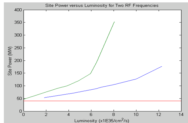
Figure 3 Site power scaling for two RF frequencies The upper curve is for 476 MHz and the lower curve 952 MHz. The power above the 40 MW horizontal line is from the overall PEP-II RF system. The currents increase with the luminosity and, thus, increase the power usage.
