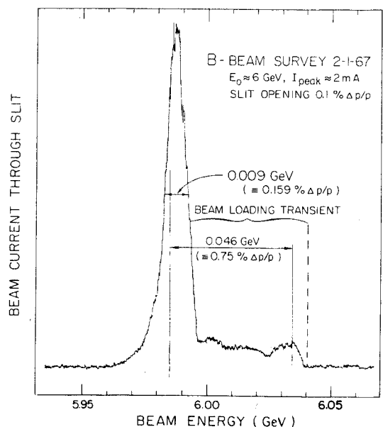
FIG. 7--Momentum spectrum of 6-GeV electron beam.
