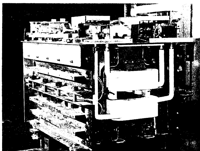
FIG. 5--0.1 0 pulsed magnet.
