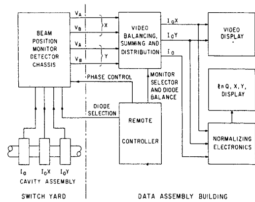
Fig. 4--Switchyard beam position monitor system
