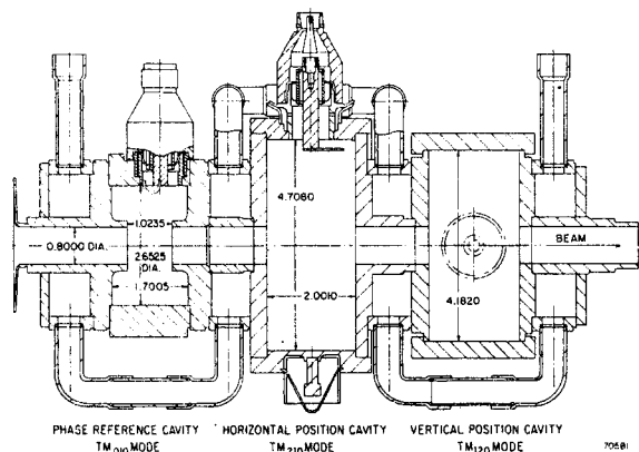
Fig. 3--In-line monitor cavity assembly
