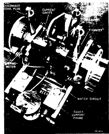
Fig. 5--Switchyard position monitor
