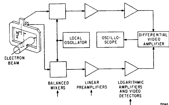
Fig. 6--End station beam position monitor system
