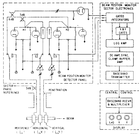
Fig. 2--In-line beam position monitor system
