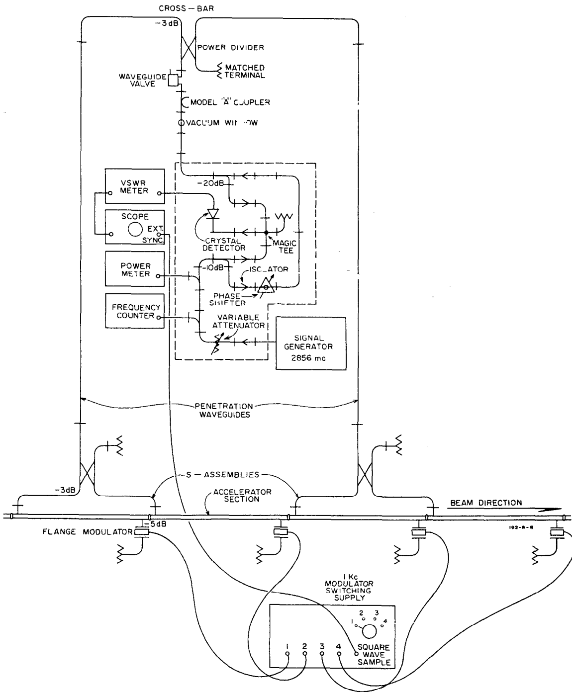
FIG. 1 - MODULATED-REFLECTION PHASE TUNING AND MEASUREMENT SYSTEM
