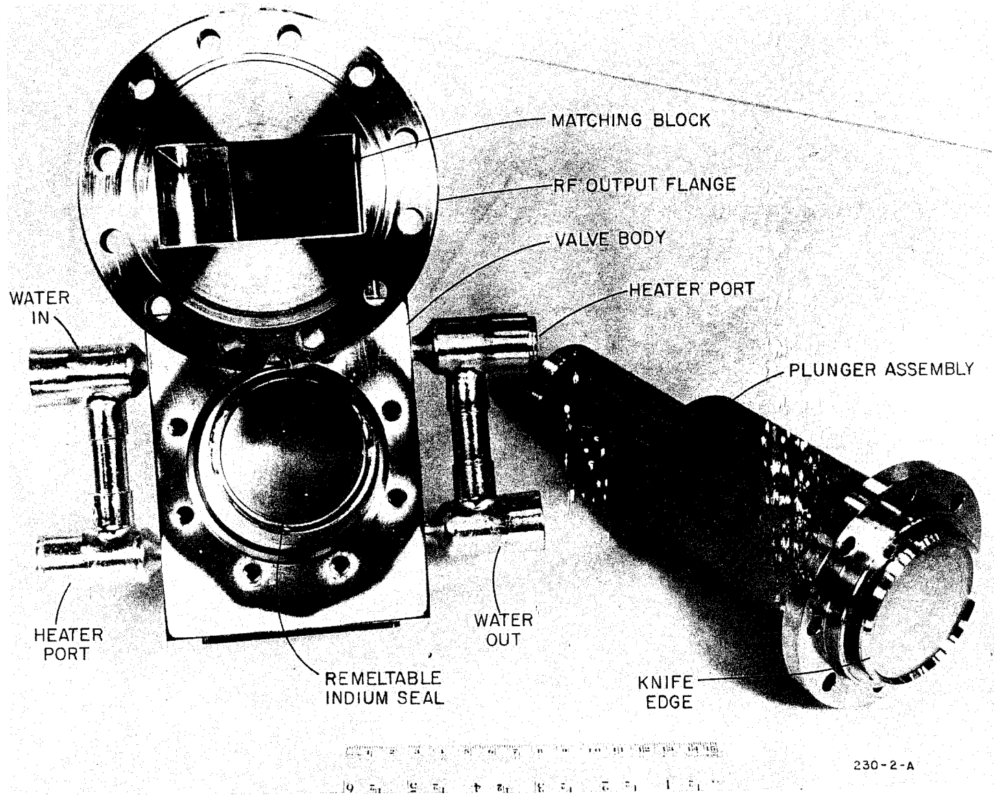
FIG. 1 - RF VACUUM VALVE, PARTIALLY DISASSEMBLED
