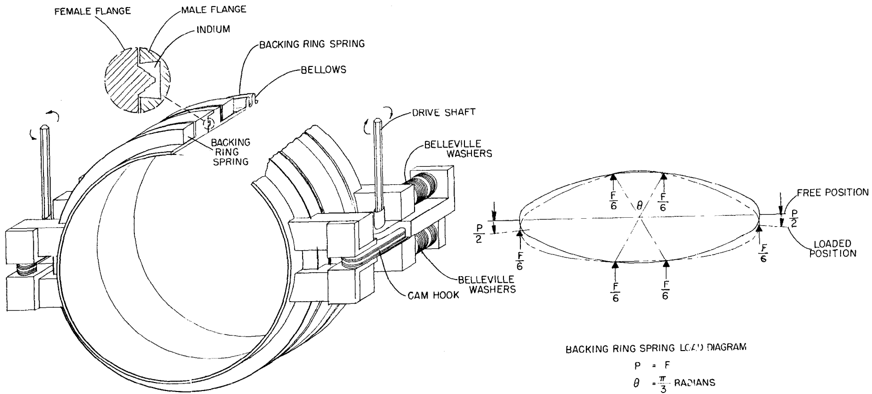
QUICK DISCONNECT VACUUM COUPLING
