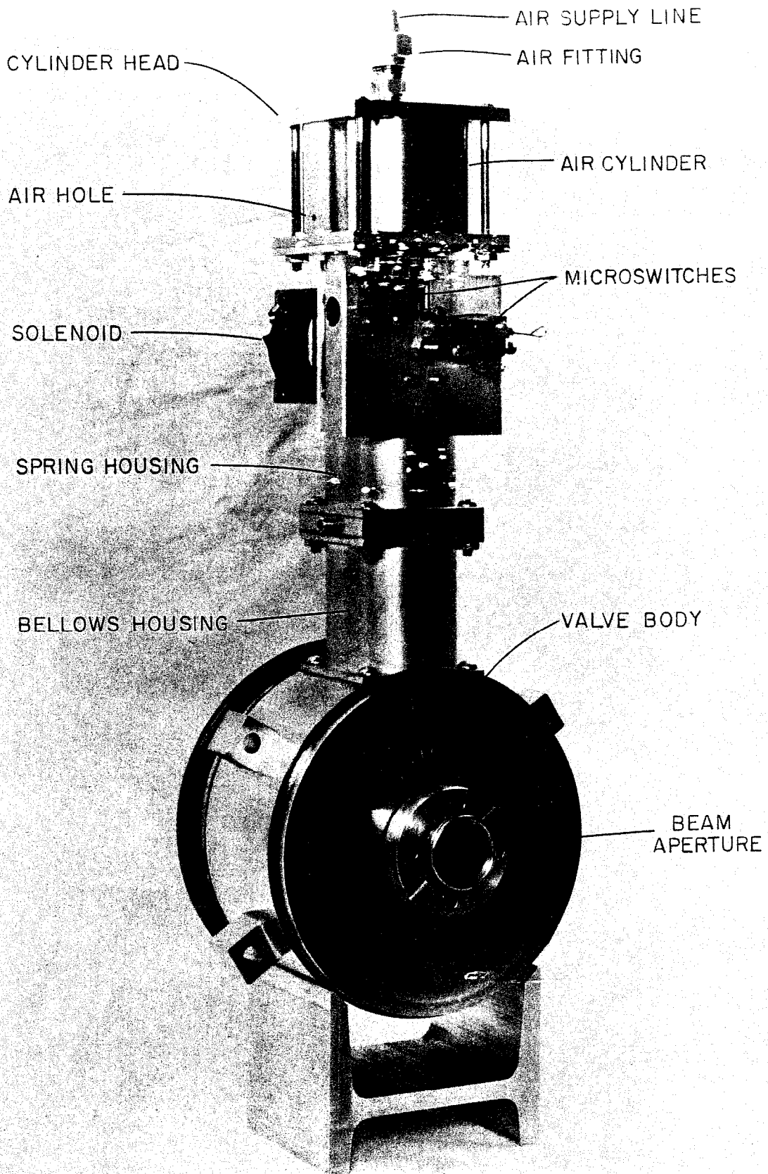
FIG. 3 - ASSEMBLED FAST CLOSING VACUUM VALVE
