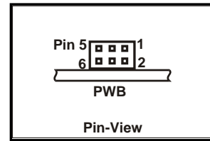
Figure 3.9-1. Auxiliary Sync Header
