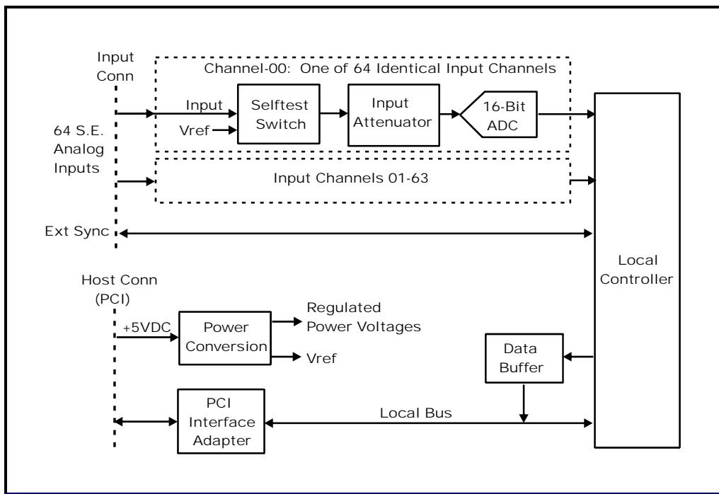
Figure 1.2-1. Functional Organization
