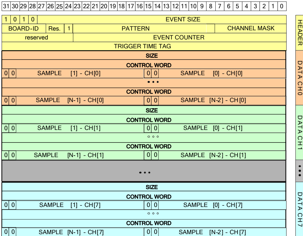
Fig. 3.9: Event Organization
