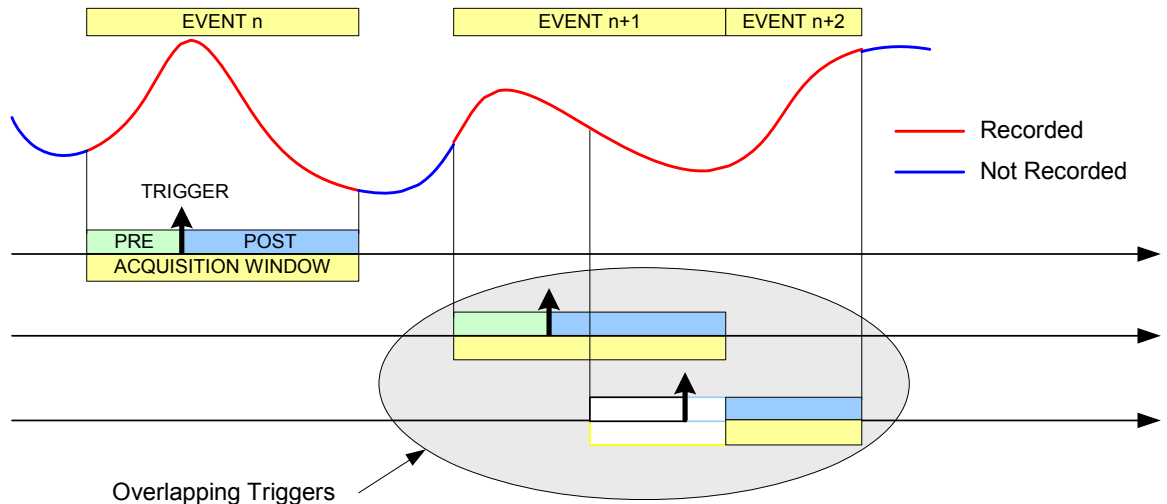
Fig. 3.8: Trigger Overlap
