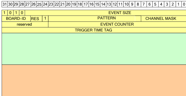
Fig. 3.11: Zero Length Encoding samples storage
