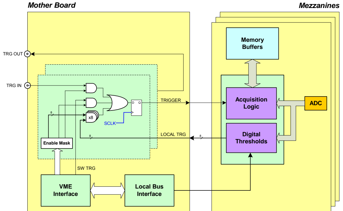
Fig. 3.17: Block diagram of Trigger management
