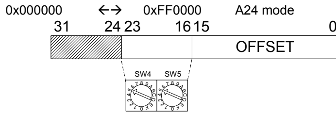
Fig. 3.25: A24 addressing
