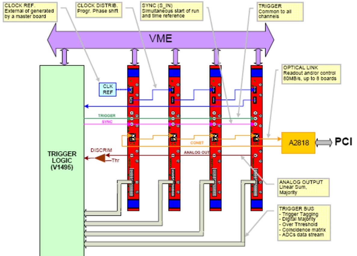
Fig. 3.20: Trigger integration
