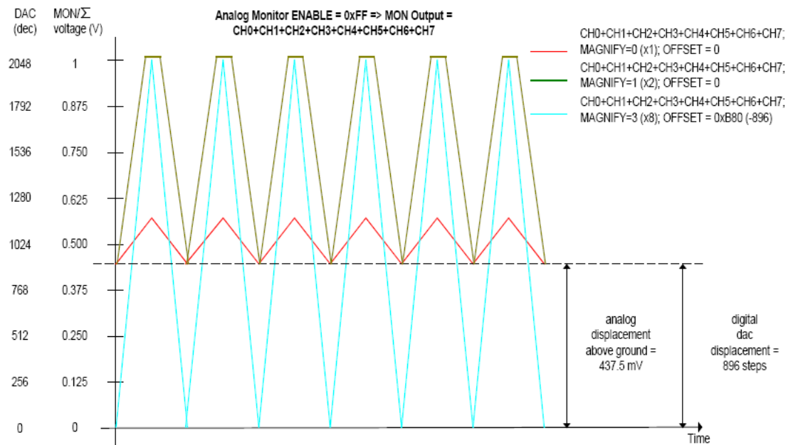
Fig. 3.24: Example of Magnify and Offset parameters use on single channel
