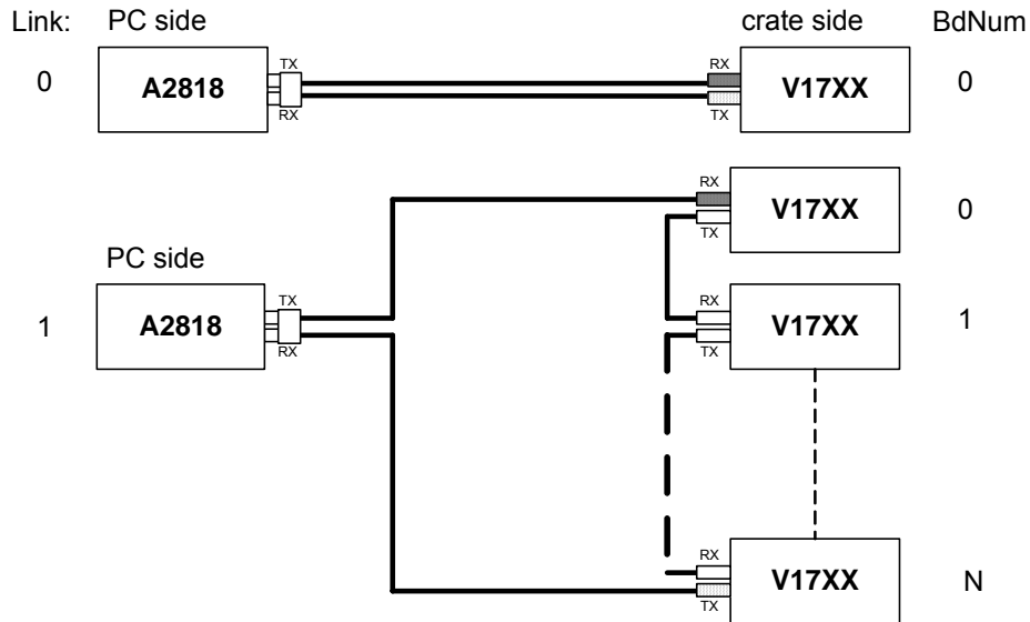
Fig. 3.31: Optical Link daisy chain
