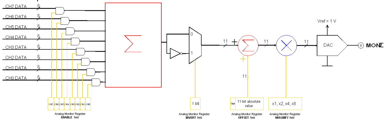
Fig. 3.22: Inspection Mode diagram
