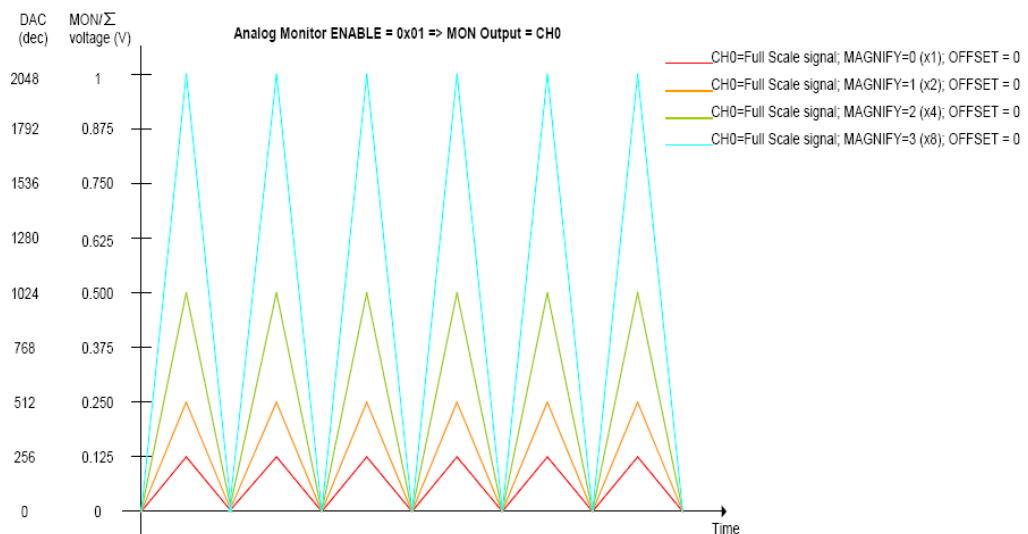
Fig. 3.23: Example of Magnify parameter use on single channel
