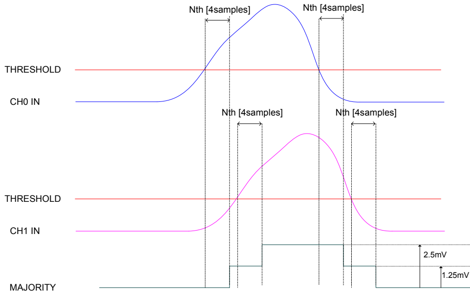
Fig. 3.21: Majority logic (2 channels over threshold; bit[6] of Ch. Config. Register =0)
