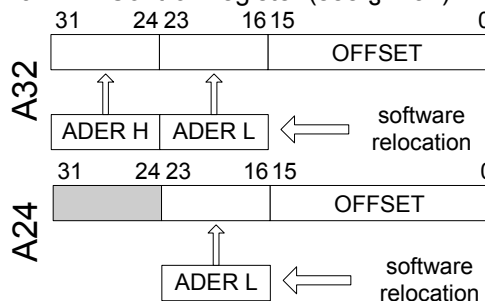
Fig. 3.28: Software relocation of base address
