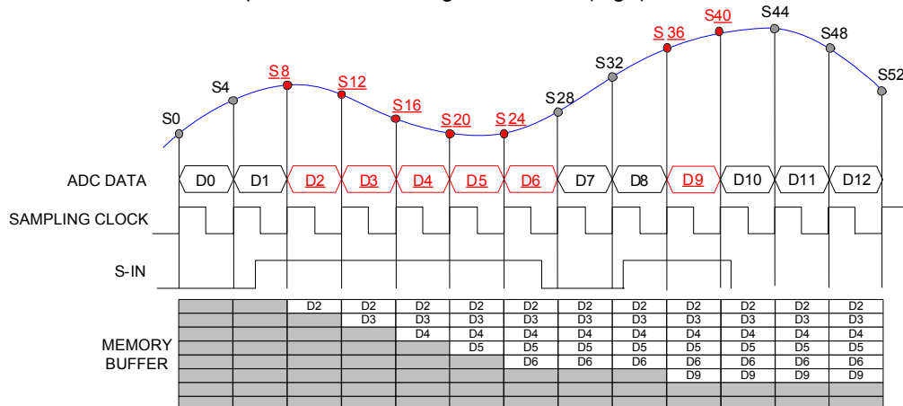
Fig. 3.6: Data Storage 1 in Gate mode
