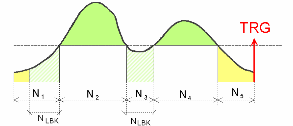
Fig. 3.16: Example with positive logic and overlapping N_{LBK}
