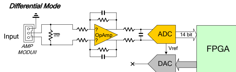
Fig. 3.2: Differential input diagram
