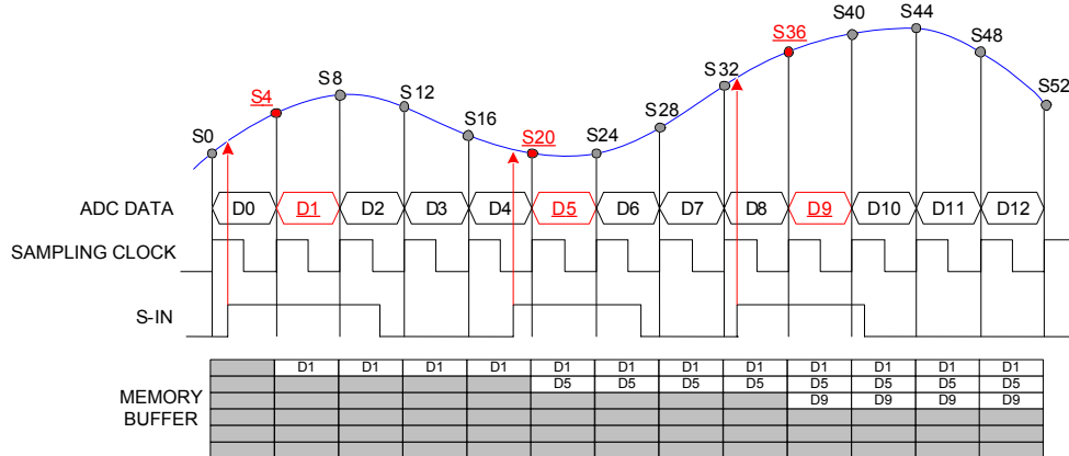
Fig. 3.7: Data storage 2 in Sample Mode
