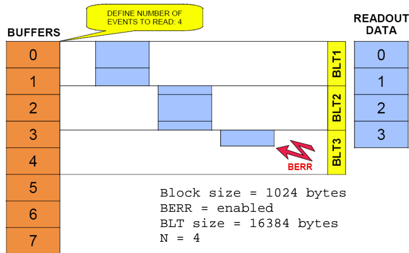
Fig. 3.29: Example of BLT readout
