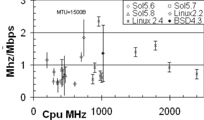
Figure 3: Ratio of measurement host MHz utilization to Mbits/s transferred
