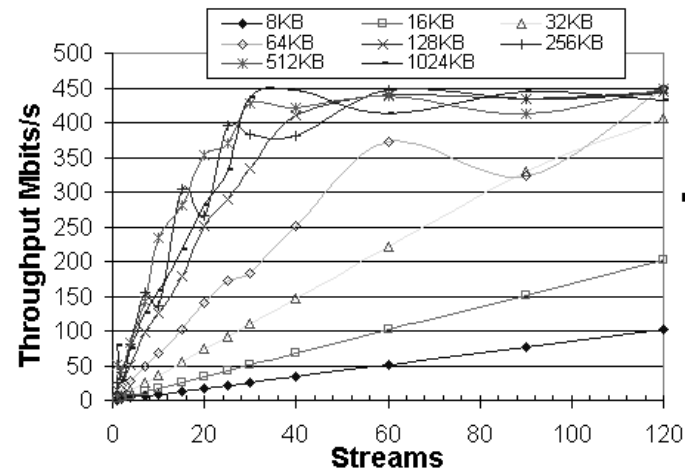
Figure 4: Ten second iperf TCP throughputs from SLAC to ANL
