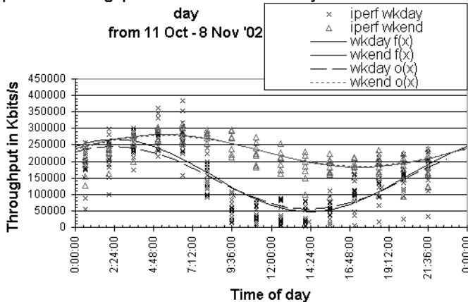
Figure 12: Iperf TCP diurnal variations
