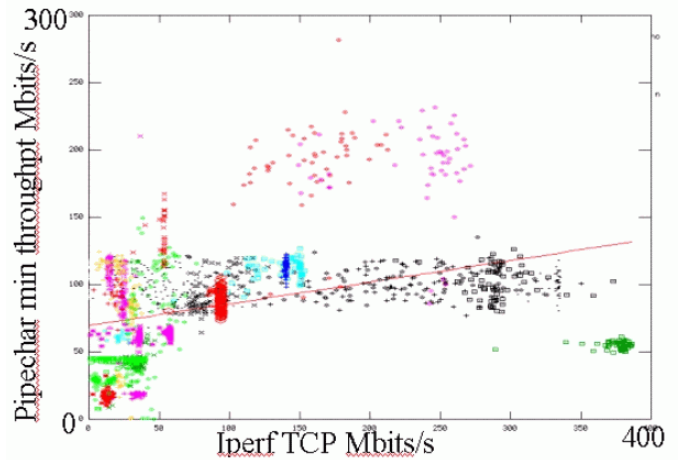
Figure 7: Pipechar estimates vs. iperf TCP throughput
