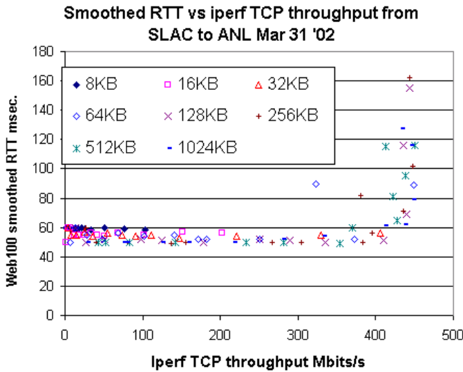
Figure 6: Web100 smoothed RTT vs. iperf TCP throughput from SLAC to ANL, Mar 31 2002.
