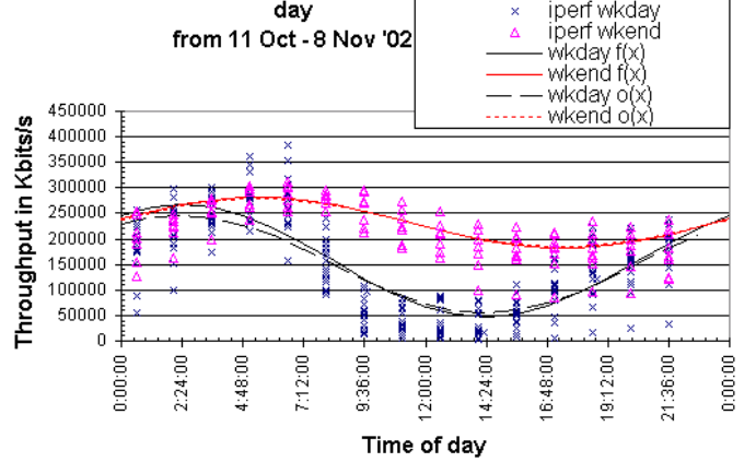
Figure 11: Iperf TCP diurnal variations
