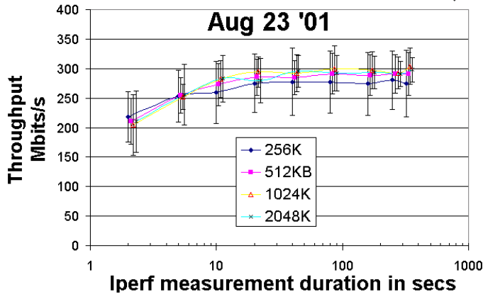
Figure 2: Iperf TCP throughput by measurement duration from SLAC to Caltech, Aug 23 2001
