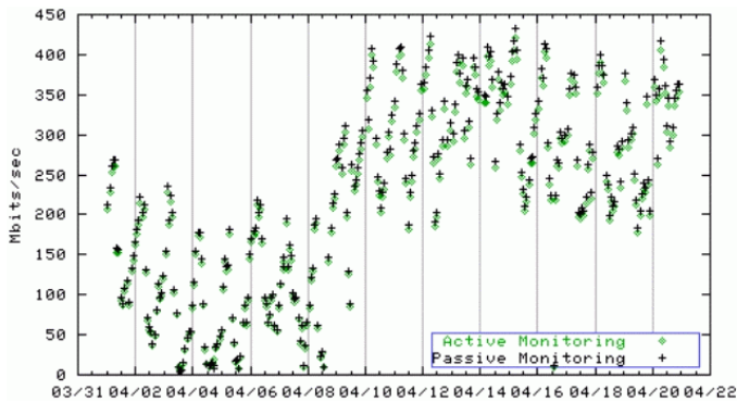
Figure 12: Example of time series of active and passive throughputs from SLAC to Caltech, Mar-Apr 2002
