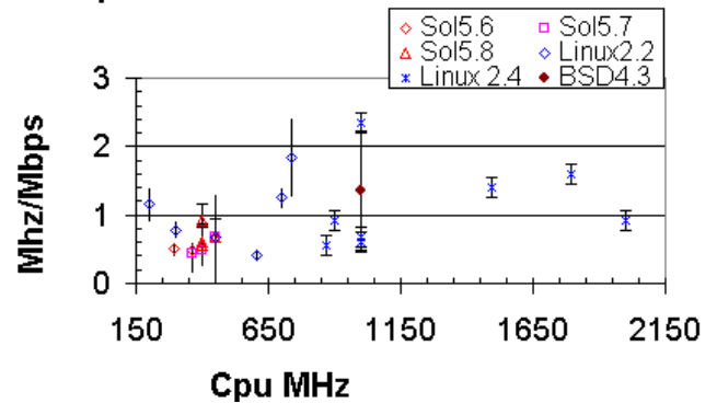
Figure 3: Ratio of measurement host MHz utilization to Mbits/s transferred
