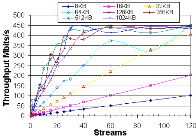
Figure 4: Ten second iperf TCP throughputs from SLAC to ANL
