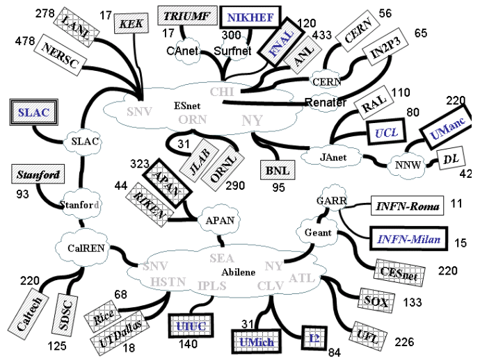
Figure 1: Routes and iperf TCP Mbits/s from SLAC to the remote sites.
