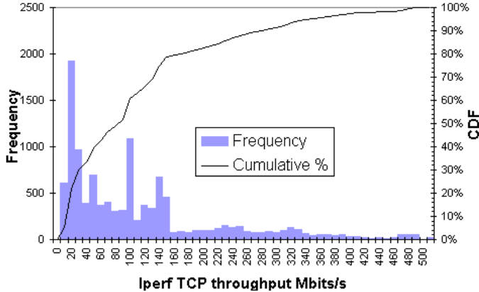
Figure 9: Iperf TCP throughput frequency histogram.
