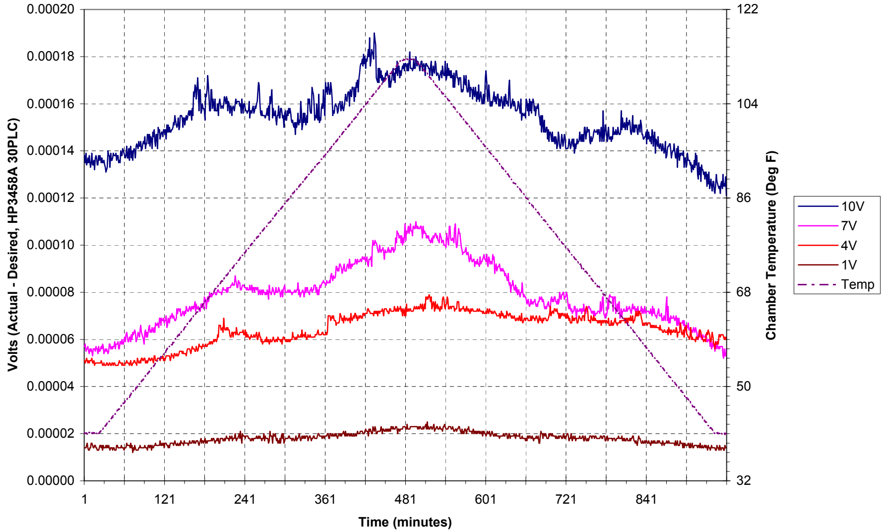
EPSC DAC Stability vs Temperature (5C to 45C to 5C)
