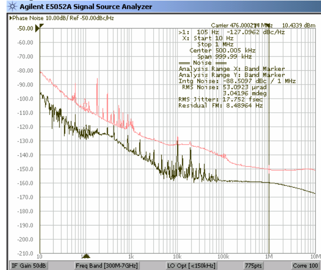
Figure 3: Phase noise spectrum of the LCLS oscillator, bottom, compared to Linac RF, Top 10 Hz to 10 MHz.
