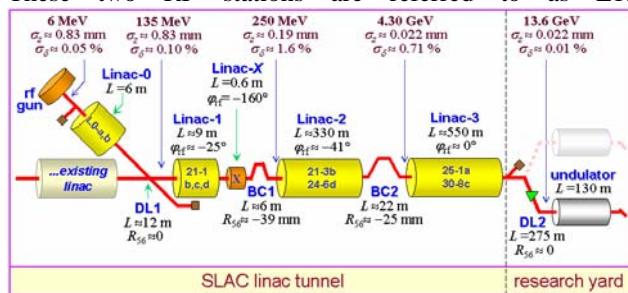
Figure 1 : LCLS Layout
