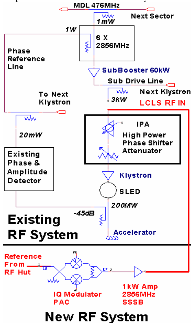
Figure 4: SLAC Linac RF System and LCLS Input.
