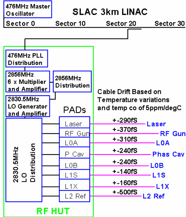
Figure 2: Reference and Signal Cables.
