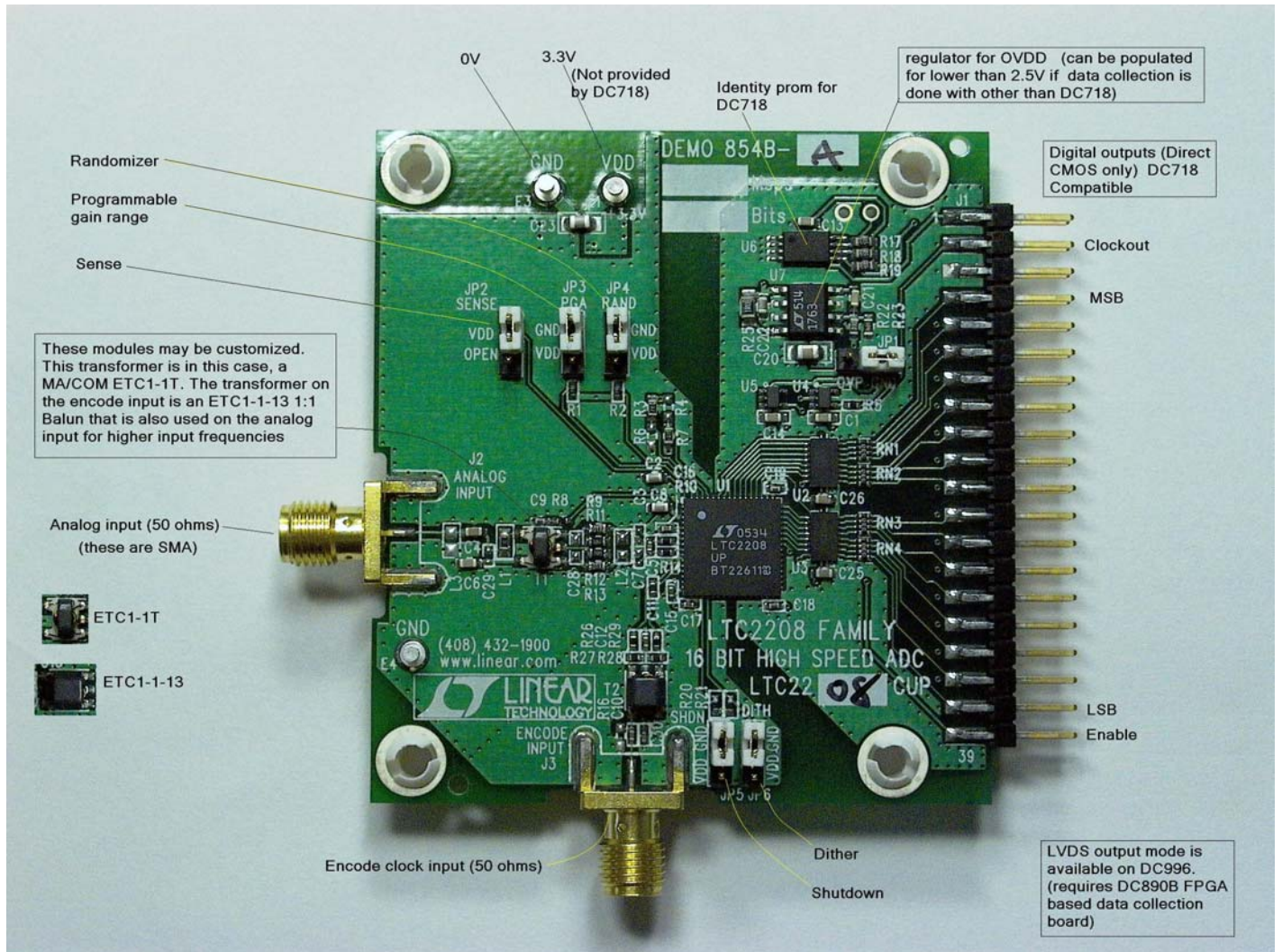
Figure 1. DC854 Setup (zoom for detail)
