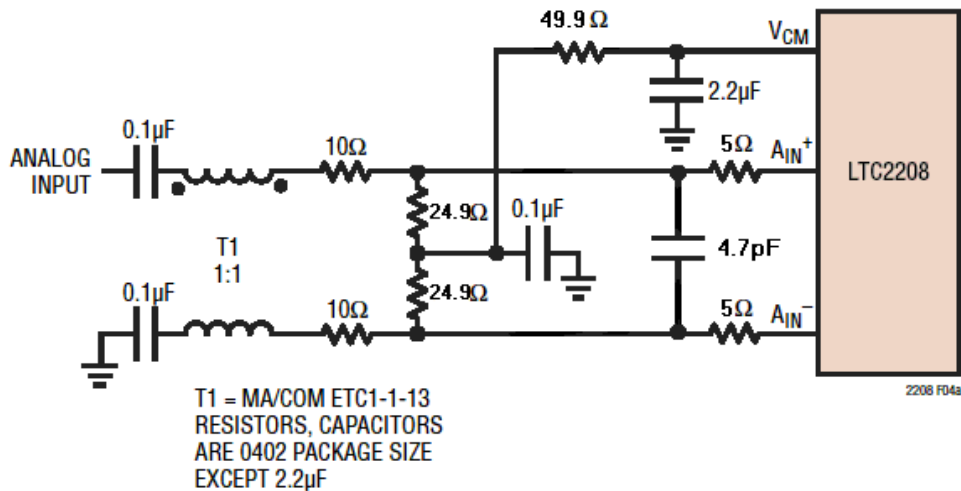
Figure 2. Analog Front End Circuit For 70MHz+
