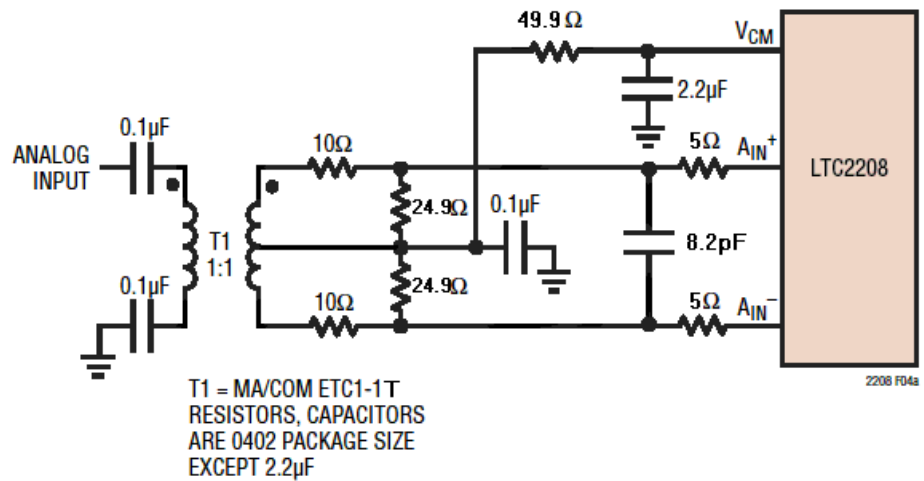
Figure 2. Analog Front End Circuit For 70MHz+
