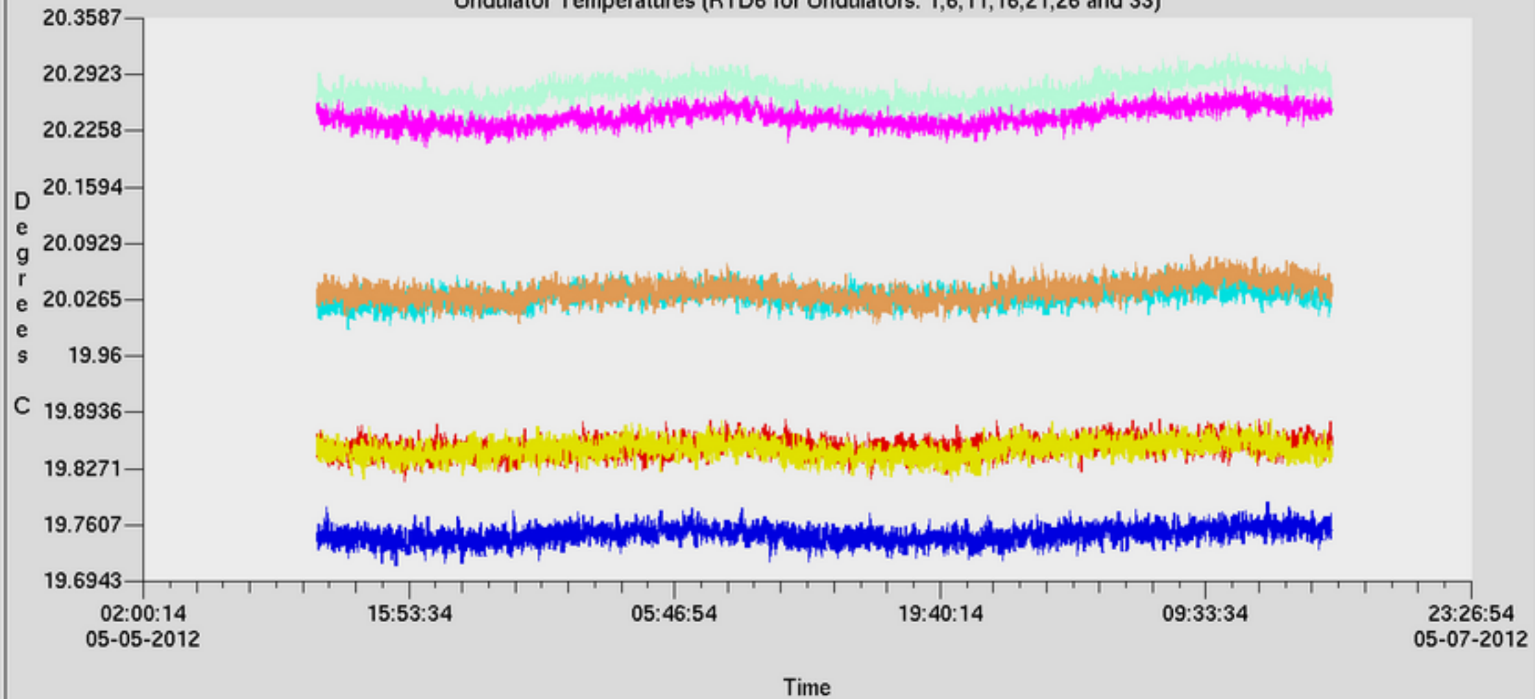
Undulator Temperatures (RTD6 for Undulators: 1,6,11,16,21,26 and 33)
