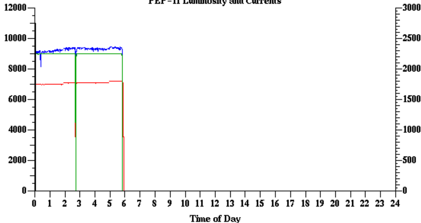
PEP-II Luminosity and Currents
