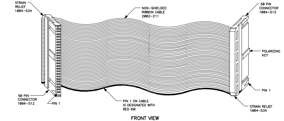
MODEL 5025-550-x SIGNAL CABLE, NON-SHIELDED
