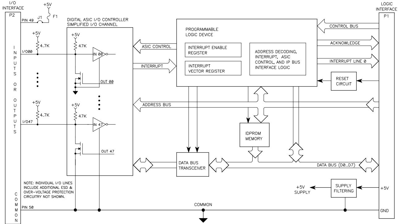
IP470 BLOCK DIAGRAM
