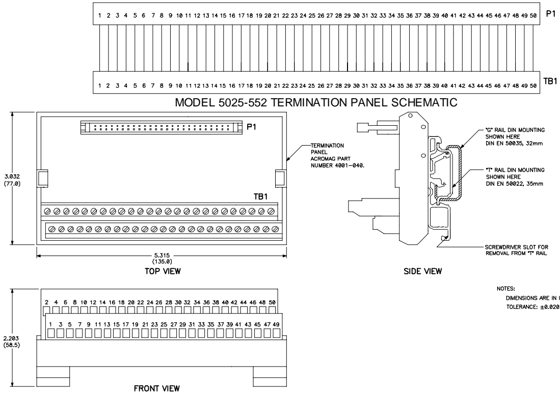
MODEL 5025-552 TERMINATION PANEL
