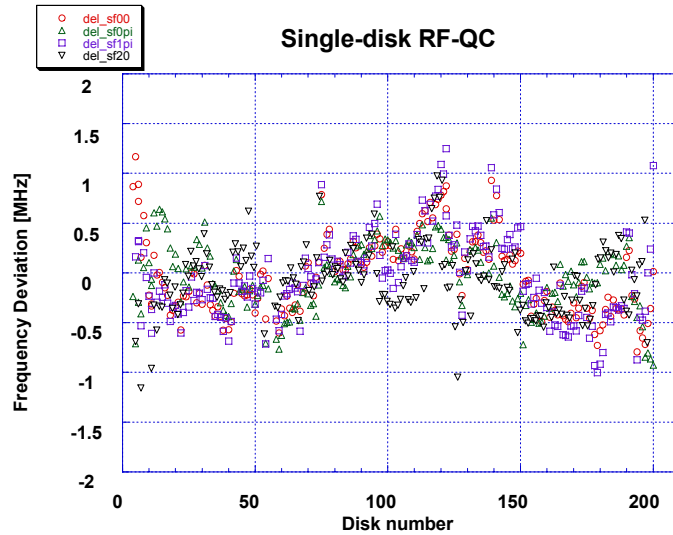
Figure 14. Four frequencies measured in a single-cell QC setup versus cell number.
