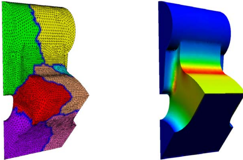
Figure 3. Meshes for parallel modeling (left) and illustration of pulse heating (right).
