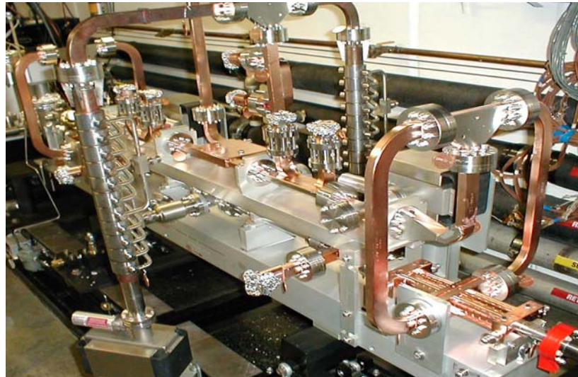
Figure 11. A pair of SW structures installed in the NLCTA beamline.
