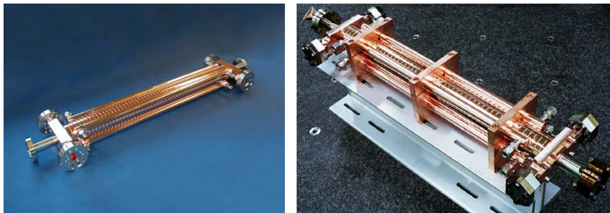
Figure 15. Recent 60 cm-long structure made by SLAC (left) and KEK (right).
