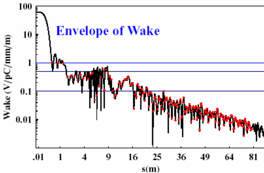
Figure 5. Calculated wakefield for recently designed HDDS structure. The dots indicate the locations of the bunches, which have a 1.4 ns spacing.
