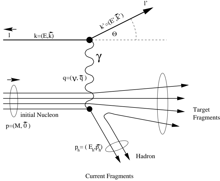
Figure 6. A schematic illustration of the hadronization process.
