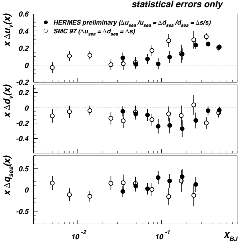
Figure 10. Preliminary data on the quark spin distributions at the measured Q^2 are shown separately for the valence \Delta u_v , \Delta d_v and the sea \Delta \bar{u} as a function of x . The error bars shown are statistical only. The distributions are compared to results from SMC evolved to Q^2 = 10 \text{ GeV}^2 . The error bars of the SMC result correspond to its total uncertainty.
