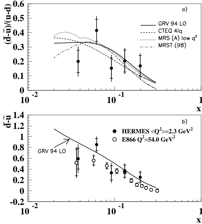
Figure 11. In the top panel, (\bar{d} - \bar{u})/(u - d) as a function of x is shown. Also included are GRV 94 LO, 27 CTEQ 4lq, 28 MRS (A) 29 low Q^2 , and MRST (98) 30 parameterizations calculated at the appropriate Q^2 for each x -bin. In the bottom panel (\bar{d} - \bar{u}) as a function of x is shown. The curve is the GRV 94 LO parameterization. The E866 data determined from (\bar{d} - \bar{u}) are represented by open circles.
