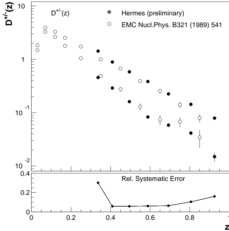
Figure 7. Preliminary data on the favored D^+ and disfavored D^- pion fragmentation functions from HERMES are compared to data from EMC. They are shown in the top panel. The same extraction method has been used for both data sets. The relative systematic errors are displayed in the lower panel.
