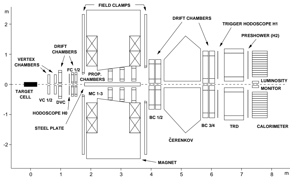
Figure 3. Schematic side view of the HERMES spectrometer.
