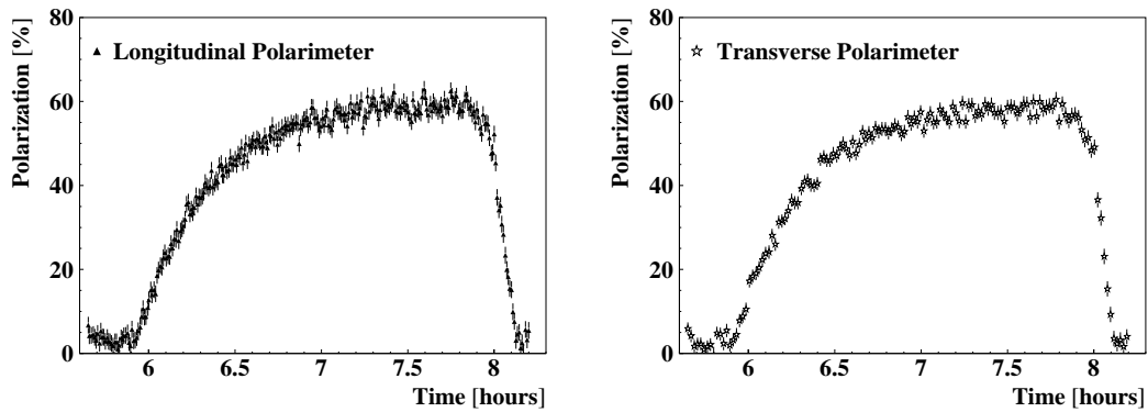
Figure 1. Polarization rise time recorded simultaneously with the longitudinal and transverse polarimeters to compare build-up time and general performance of both polarimeters. At the beginning and the end of the spectrum, the beam was depolarized on purpose.
