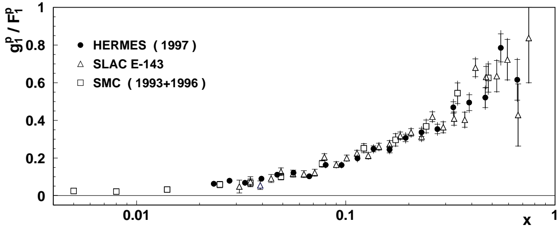
Figure 4. The structure function ratio g_1^p / F_1^p of the proton as a function of x from HERMES is compared with recent results for g_1^p / F_1^p measured at SLAC (E143) and A_1^p at CERN (SMC). The inner error bars show the statistical uncertainties and the outer ones the quadratic sum of the statistical and total systematic uncertainties.
