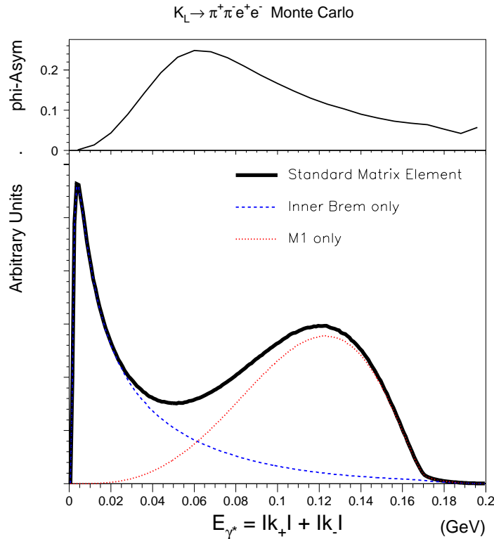
Fig. 4. The predicted angular asymmetry is shown as a function of the virtual photon energy in the kaon rest frame (top). The bottom plot shows the contributions to the matrix element from inner brems and direct emission amplitudes.
