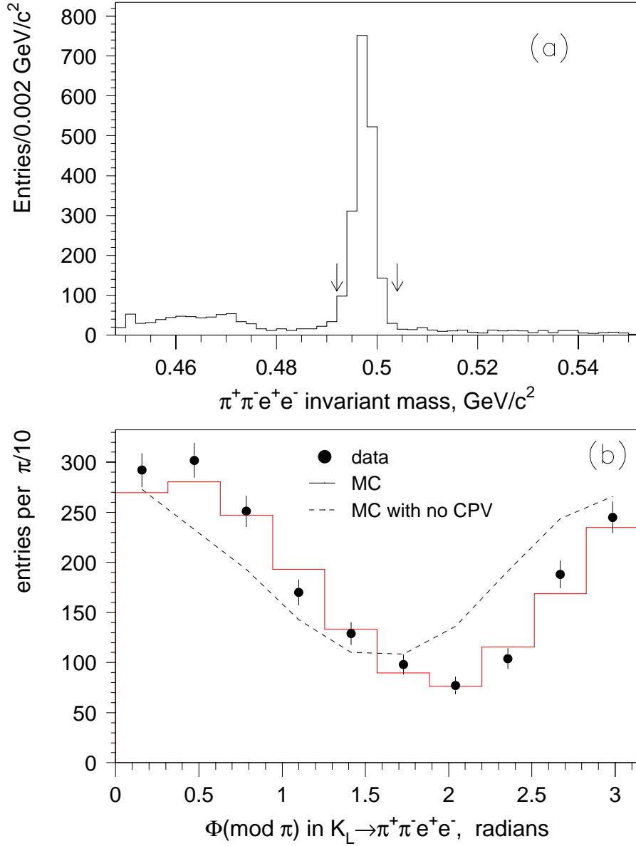
Fig. 6. Our preliminary \pi^+\pi^-e^+e^- invariant mass spectrum is shown in (a) after all analysis cuts. The arrows show the mass window (0.492 to 0.504 \text{GeV}/c^2 ) used to select K_L \rightarrow \pi^+\pi^-e^+e^- events for the angular distribution shown in (b). Events at \phi and \phi + \pi are plotted in the same bin. The dots are for data, the histogram is the Monte Carlo using the standard model matrix element, and the dashed curve is a Monte Carlo with no CP-violation in the matrix element.
