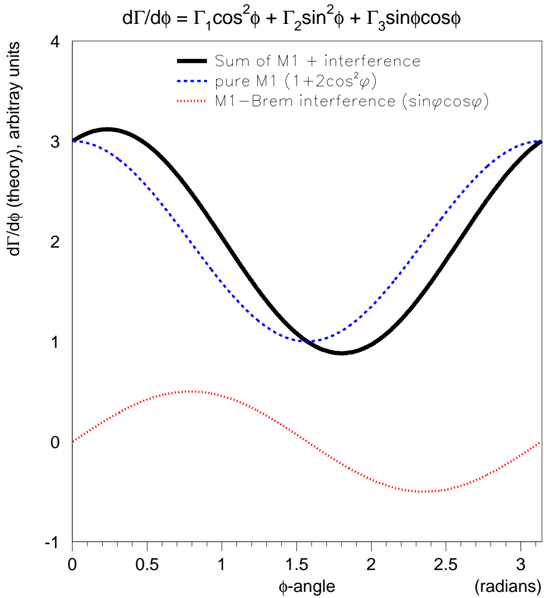
Fig. 5. The predicted \phi distribution is shown for M1 direct emission (dashed), M1-brem interference (dots) and the sum of M1 and interference (solid).
