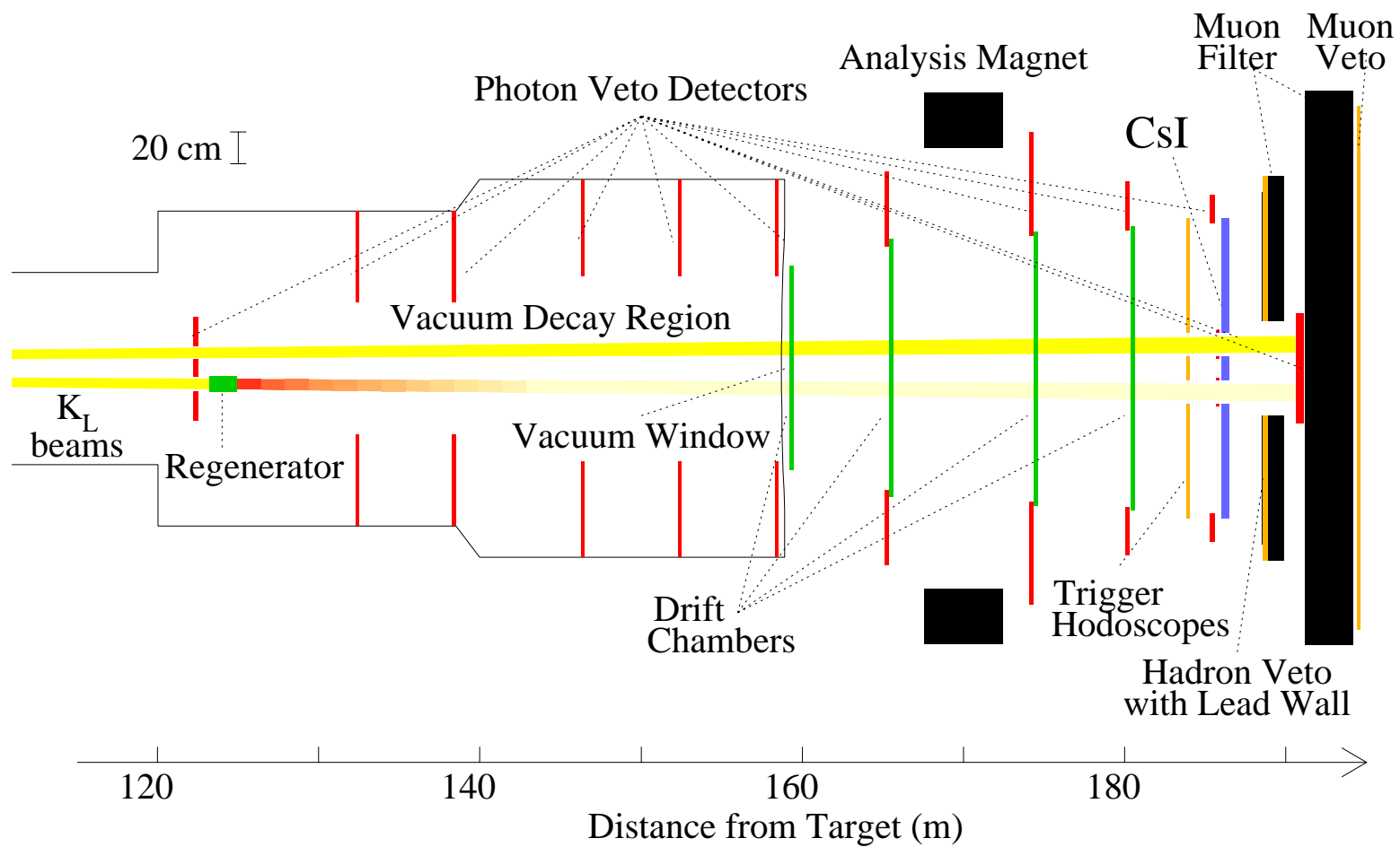
Fig. 1. The KTeV detector configuration used for the measurement of \text{Re}(\epsilon'/\epsilon) .
