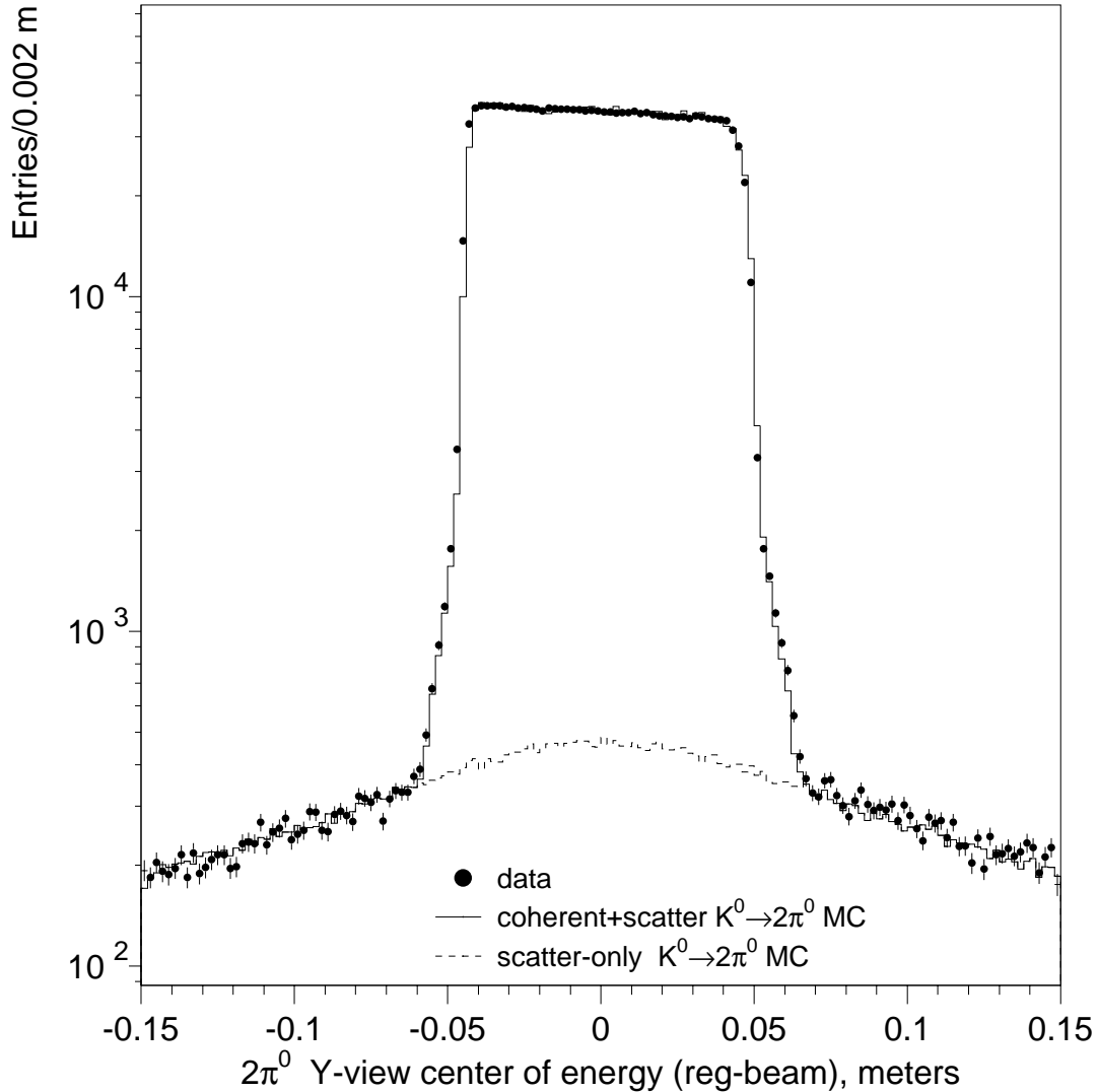
Fig. 3. Preliminary four-photon center of energy (meters) in the Y -view is shown for 2\pi^0 decays in the regenerator beam. All other off-line analysis cuts have been applied, including a cut on the X -view center of energy. The data are shown by the solid dots. The dashed histogram is from a background Monte Carlo simulation of kaon scatters in the regenerator. The histogram overlay is the Monte Carlo background (dashed) plus the coherent signal.
