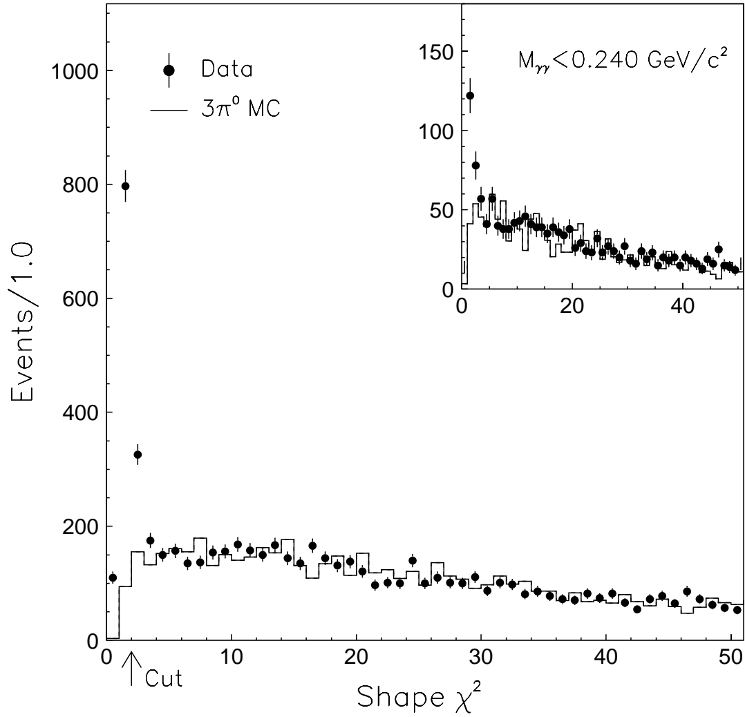
Fig. 7. The maximum transverse shape \chi^2 of the four photons for each K_L \rightarrow \pi^0\gamma\gamma candidate after all off-line software cuts except the \chi^2 cut ( preliminary ). The inset shows the same distribution for events with m_{\gamma\gamma} < 0.240 \text{ GeV}/c^2 . The data are shown by dots; the histogram is from a Monte Carlo simulation of K_L \rightarrow 3\pi^0 events.
