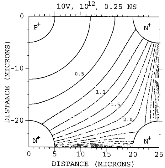
Fig. 6. Lines of equal drift time for potential distributions of Fig. 2(c) ( 10^{12}/\text{cc} and 10\ \text{V} ). Zero time is measured from the p^+ -electrode (top left corner) at r = 5\ \mu\text{m} and charges are traced backwards. Lines in the immediate vicinity of the zero-field points at the bottom center and right center are not reliable: diffusion plays a major role there. In addition, few of the tracks being traced backwards go there.
