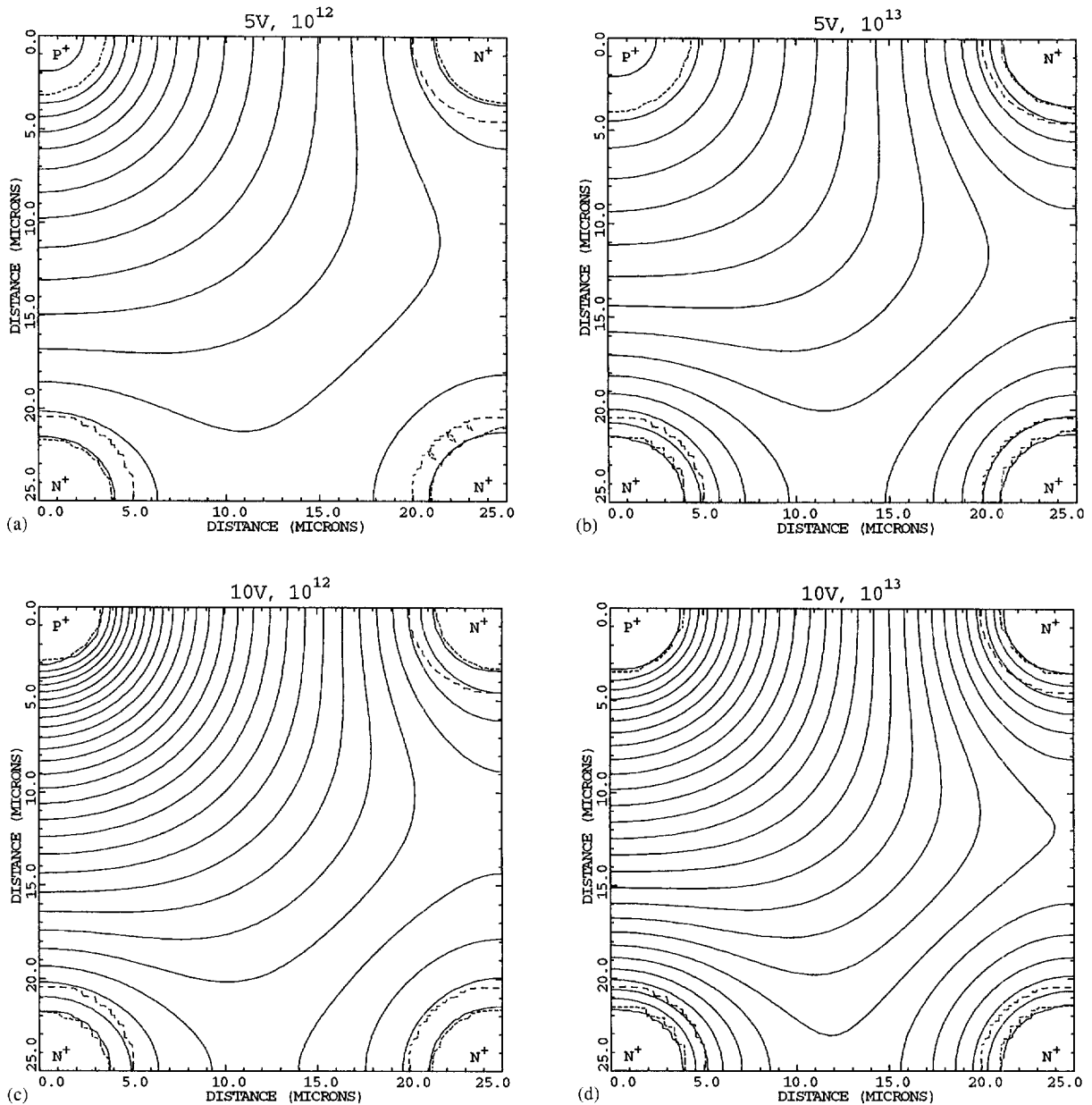
Fig. 2. (a) Equipotentials for one quarter of the unit cell of Fig. 1 with 10^{12} dopant atoms/cc when 5 V is applied between the two electrodes. The boundaries of the depleted region are indicated by short dashes. Lines with longer dashes, mark n-p junctions; (b) equipotentials for 10^{13}/\text{cc} , 5 V; (c) for 10^{12}/\text{cc} , 10 V; (d) for 10^{13}/\text{cc} , 10 V. Effects of surface charges are not included. The lack of cylindrical symmetry in the fields and depletion depths into the electrodes, especially of the n^+ ones adjacent to the p^+ -electrode, can be seen as can the decrease in low-field volume for the heavier ( 10^{13}/\text{cc} ) substrate doping.
