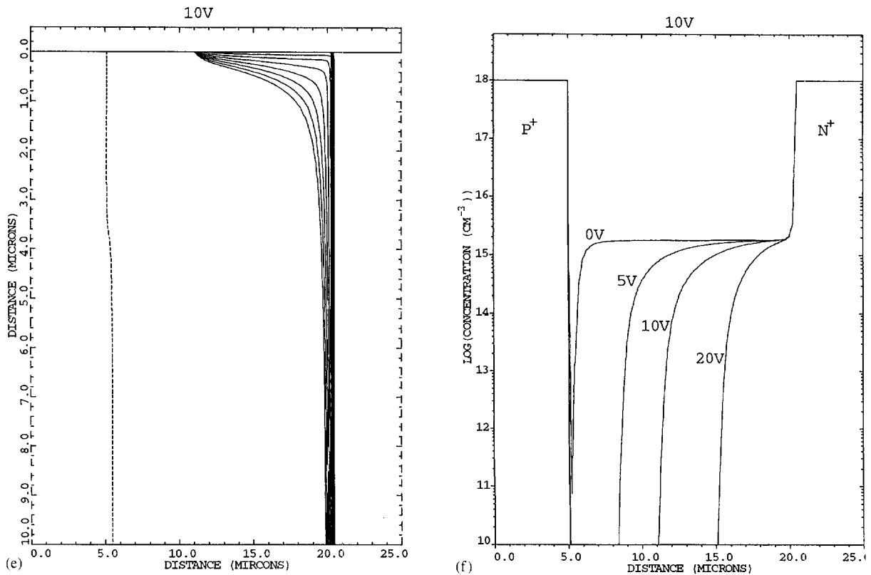
Fig. 9. Effects of an oxide interface charge of 10^{11}/\text{cm}^2 . In this two-dimensional example, the p^+ - and n^+ -electrodes are at 0–5 \mu\text{m} and 20–25 \mu\text{m} , doped throughout at 10^{18}/\text{cc} , and the charges are along the top between them. The substrate doping is 10^{12}/\text{cc} . (a) Applied voltage = 0 V. The effect of negative charge induced by the oxide charge can be seen with the closest equipotential almost parallel to the surface. The contact of the induced charge with the n^+ -electrode on the right forces the equipotentials from the built-in field into a bundle next to the p^+ -electrode. The capacitance between the two electrodes will be relatively high. (b) Similar equipotentials for 5 V and, (c) 10 V. An increasingly wider depletion zone at the surface can be seen. (d)–(e) Electron density contours for 0 and 10 V. (f) Net carrier concentration 0.1 \mu\text{m} below the surface for 0, 5, 10, and 20 V.
