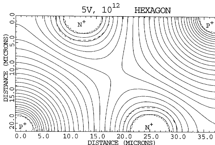
Fig. 13. Equipotentials for a cell of Fig. 10(c), 10^{12}/\text{cc} doping, 10 V.
