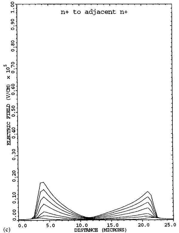
Fig. 4. Electric field magnitudes for the quarter cell of Fig. 2(a), substrate doping of 10^{12}/\text{cc} , and applied voltages of 50, 40, 30, 20, 10, 5, and 0 V (top to bottom lines) along lines from (a) the p^+ to the adjacent n^+ -electrode, (b) the p^+ to the diagonally opposite n^+ -electrode, and (c) the n^+ to the adjacent n^+ electrode.
