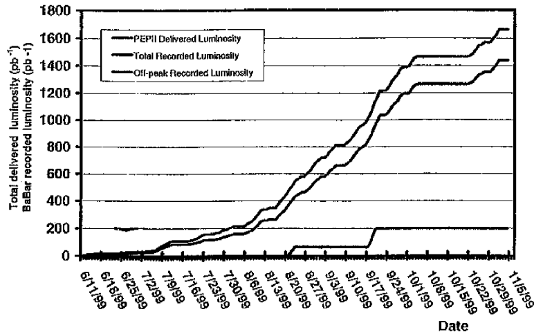
Figure 7: Integrated luminosity accumulated by PEP-II as a function of time.
