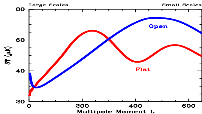
Figure 3: The spectrum of anisotropies in an open and flat universe. Plotted is the expected RMS anisotropy in micro Kelvin as a function of multipole moment. The series of peaks and troughs—the first several of which are apparent in the flat case—continues to small scales not shown in the plot. These are shifted to the right in the open case, so only the first peak shows up here. These curves are for a particular choice of cosmological parameters, corresponding to standard Cold Dark Matter.
