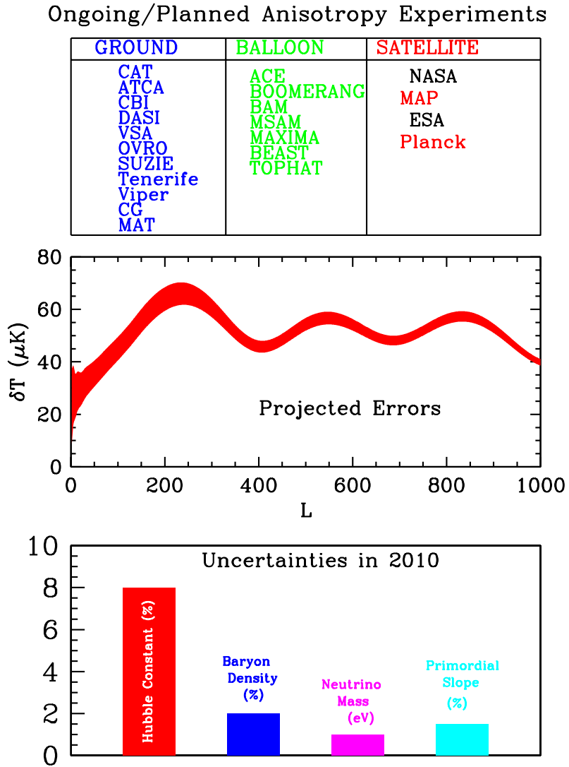
Figure 4: The future of CMB anisotropies. Top panel: Experiments expected to report anisotropy results within the next decade. Middle panel: Expected uncertainty on the anisotropy after these results come in. Bottom panel: Anticipated uncertainties in several cosmological parameters as a result of all this information.
