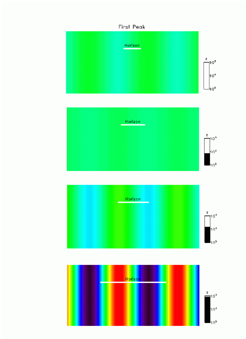
Figure 1: Four snapshots in the evolution of a Fourier mode. The top panel shows the anisotropy field to this one mode very early on, when its wavelength is still much larger than the horizon (shown as white bar throughout). The second panel, at redshift z > 10^4 shows a time at which the amplitude of the oscillations is very small. The third panel shows the amplitude getting larger; note that the hot and cold spots in the third panel are out of phase with those in the top panel. Finally, the bottom panel shows that at recombination, the amplitude has reached its peak. The side bar shows the redshift ranging from 10^5 at top to 10^3 in bottom panel.
