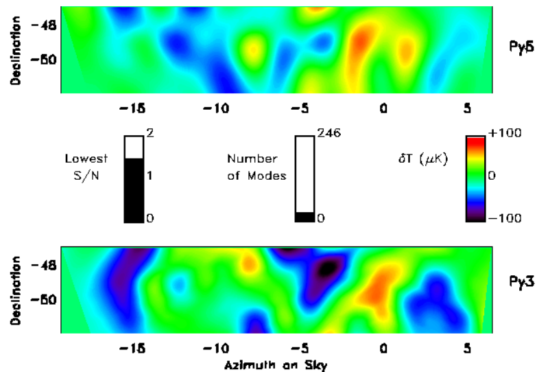
Figure 9: Two years of Python data. The bottom panel shows data from 1995; the top panel contains much noisier 1997 data. In both cases, noisy modes have been eliminated so that only modes with S/N greater than 1.5 are retained. The middle bar shows that (for Python 97) there are of order 15 such modes out of 246 pixels in the region.
