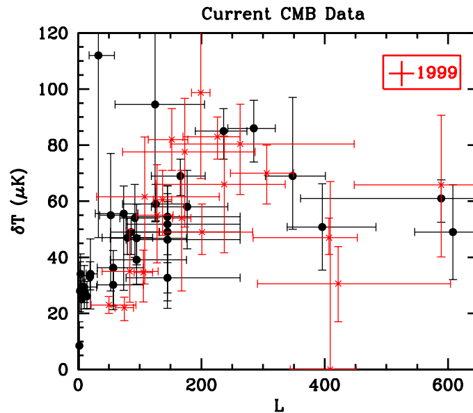
Figure 5: Current measures of CMB anisotropy. Points marked as crosses refer to measurements reported within the past year. Included are all data as of November 1999.
