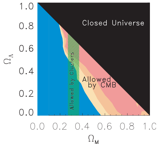
Figure 7: Constraints on the vacuum and matter densities in the universe. Shown are one-, two-, and three-sigma regions allowed by the CMB and best-fit region of the matter density from clusters.
