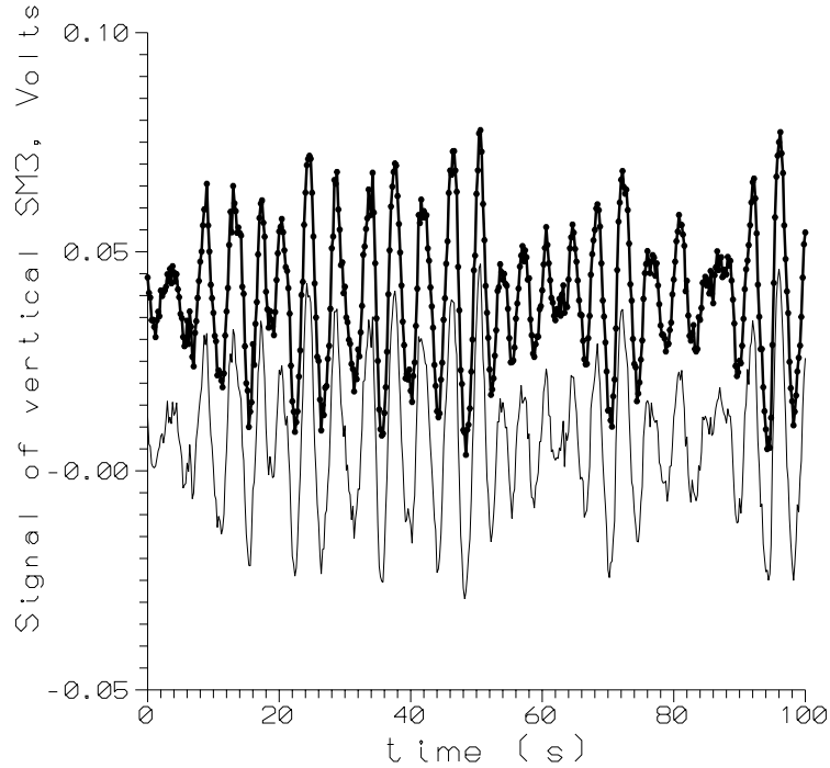
Figure 4: Signals from two vertical SM3-KV geophones separated by 32m. Measured at night of 17-18 September 1997 at E4R building.
