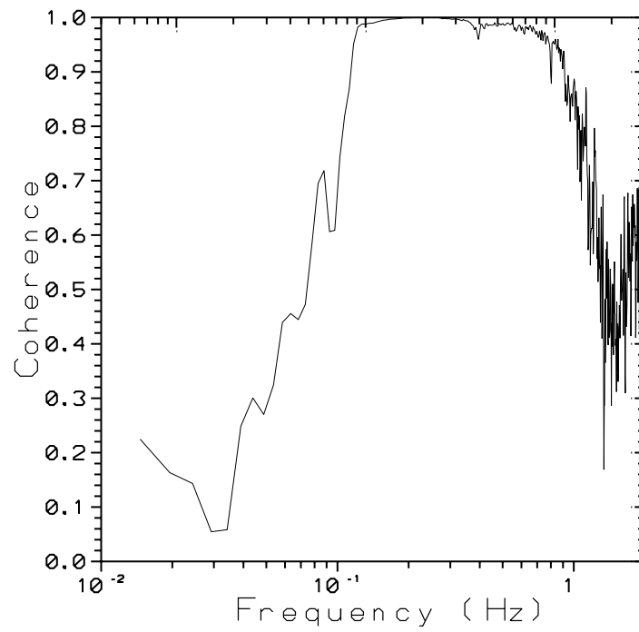
Figure 5: Coherence of vertical ground motion at distance 32 m.Night time of 09/17/97 at E4R building.
