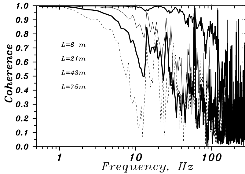
Figure 19: Coherence of the ground motion vs distance. TARP measurements.
