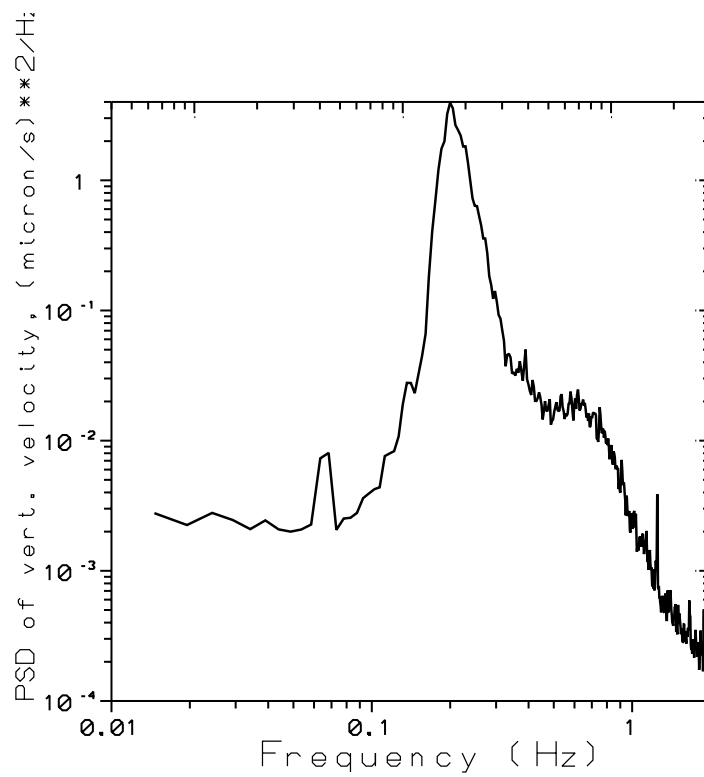
Figure 6: Power spectral density of vertical ground motion at night time.
