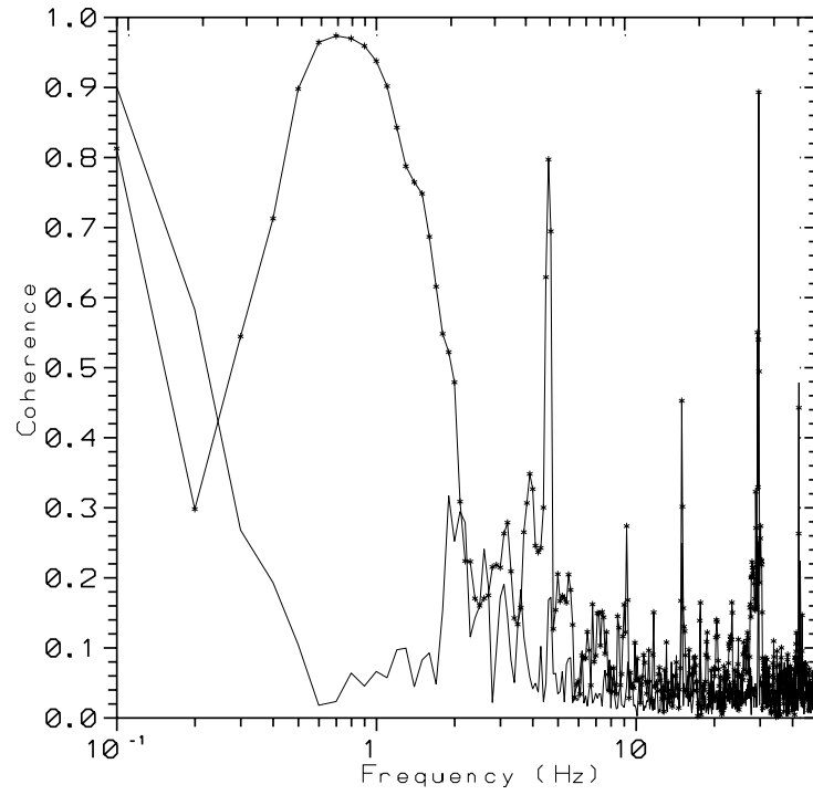
Figure 13: Coherence between signals of the vertical Tevatron beam orbit motion and the F11 magnet vibrations (marked line) and between the orbit and the tunnel floor.
