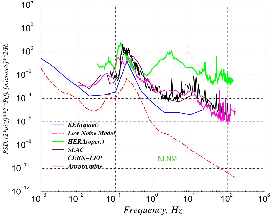
Figure 20: Ground motion spectra at different accelerator sites and the USGS New Low-Noise Model.
