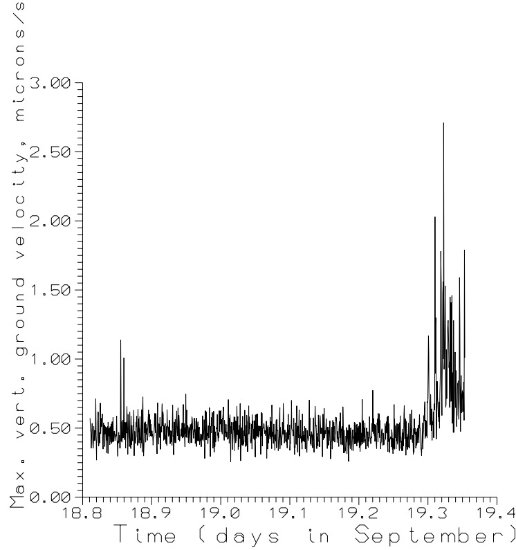
Figure 3: Maximum vertical ground velocity at E4R building recorded from 7:30 p.m. Thursday, 18 September 1997 till 8:30 a.m. 19 September 1997.
