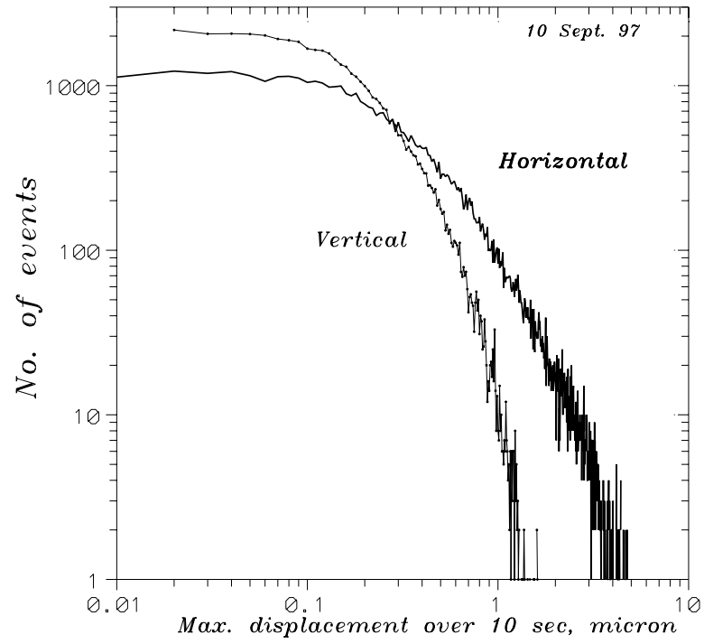
Figure 9: Distribution of maximum ground displacements over 10 s interval.
