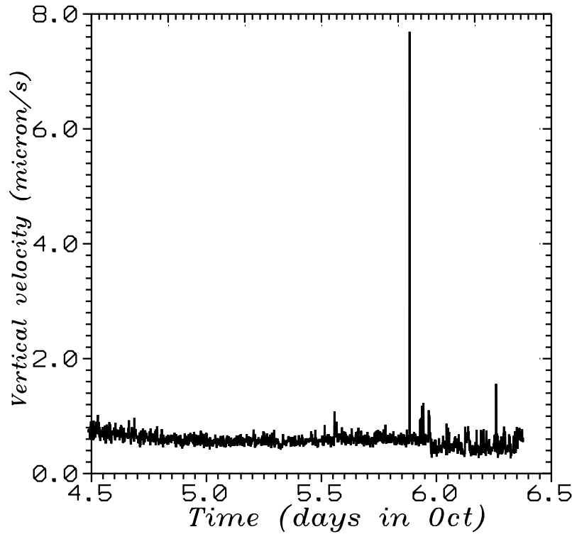
Figure 14: Maximum ground velocity in Aurora mine.
