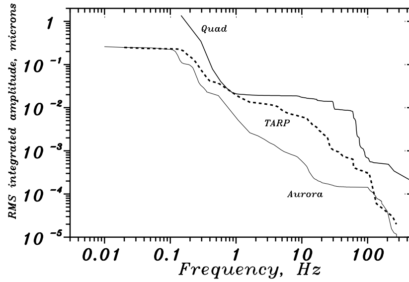
Figure 18: Integrated rms ground motion amplitude.
