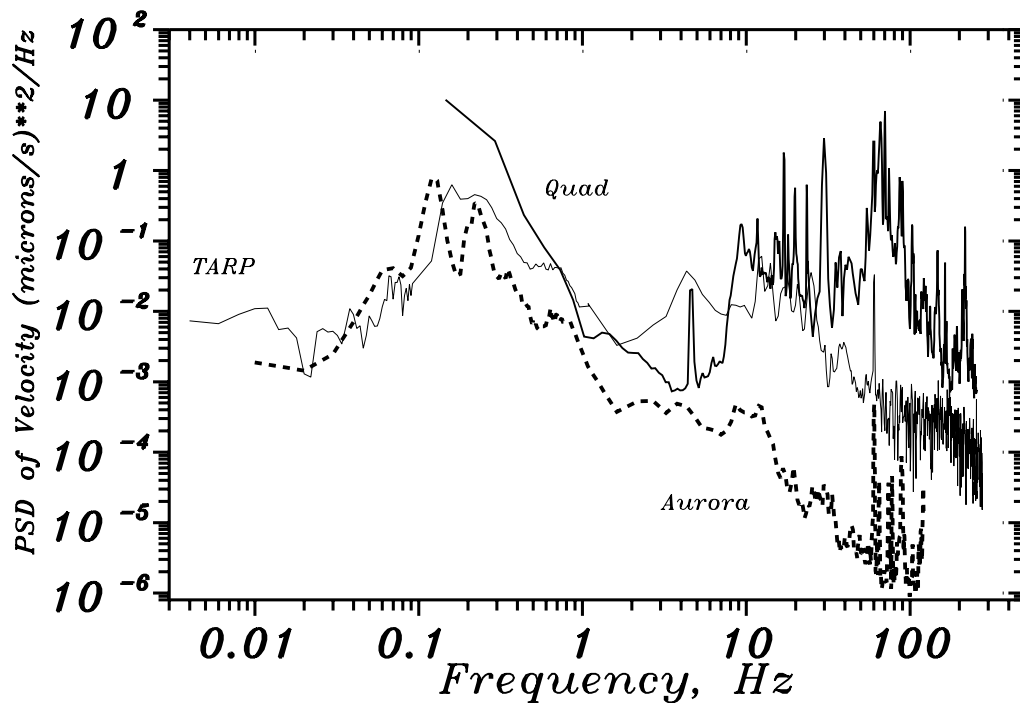
Figure 17: Spectra of ground motion in Aurora mine, TARP tunnel, and the Tevatron magnet vibrations
