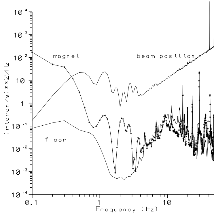
Figure 12: Spectra of the Tevatron beam orbit vibrations, tunnel floor motion and the Tevatron quadrupole vibrations at F11.
