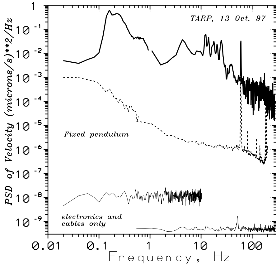
Figure 1: Typical spectrum of ground motion measured by SM3-KV probe in quiet condition (upper line), with fixed pendulum (middle) and equivalent noise of electronics only (two lower curves).
