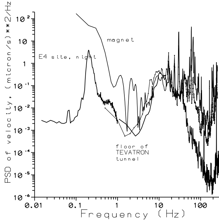
Figure 11: Power spectral densities of vertical vibrations of the Tevatron quadrupole magnet (upper curve), the tunnel floor (middle line with marks) and on the surface at E4 (lower curve).
