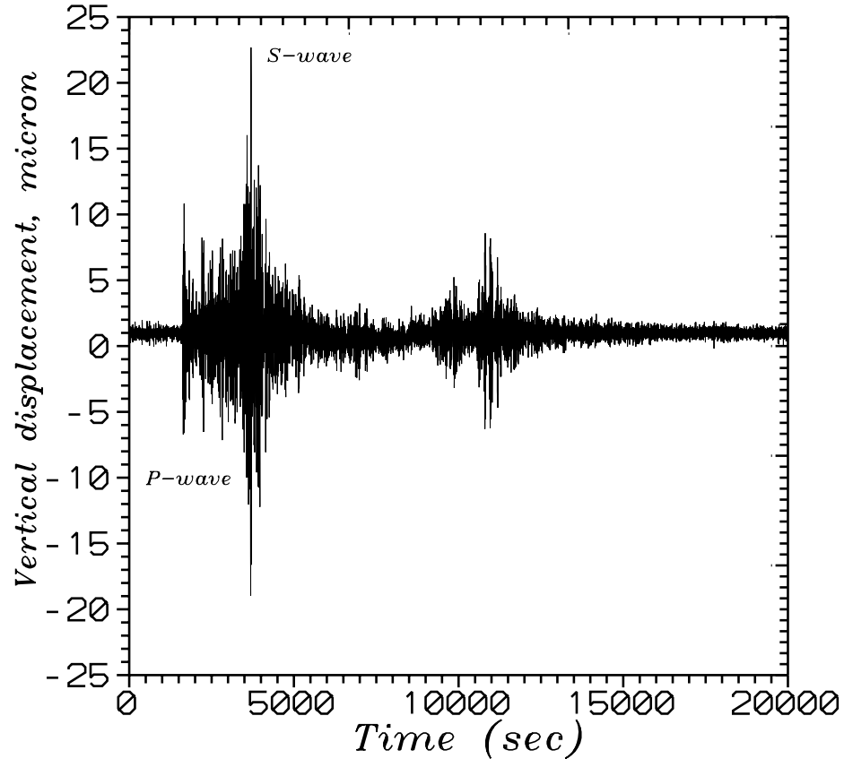
Figure 16: Earthquake waves. Record starts at 7:45 pm 10/14/97.
