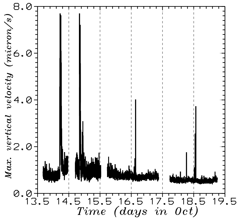
Figure 15: Maximum ground velocity in TARP shaft.
