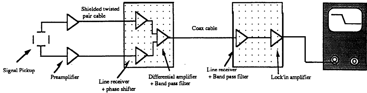
Fig. 3 A schematic of the front end electronics
