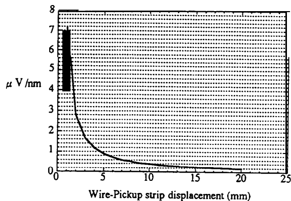
Fig. 2 The change of the sinusoidal wave amplitude at the output of preamplifier equivalent for the 1 nm movement as a function of wire-pickup strip displacement.
