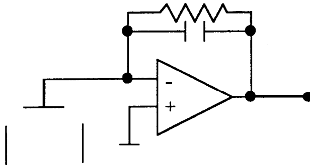
Fig. 4 Preamplifier circuit
