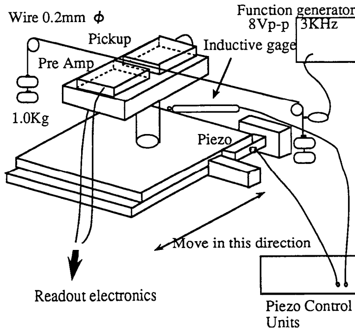
Fig. 5 The bench test setup for stretched wire alignment
