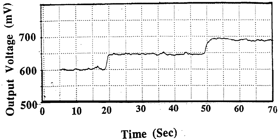
Fig. 7 The lock'in amplifier output voltage change when the monitor position is changed 50 nm step.
