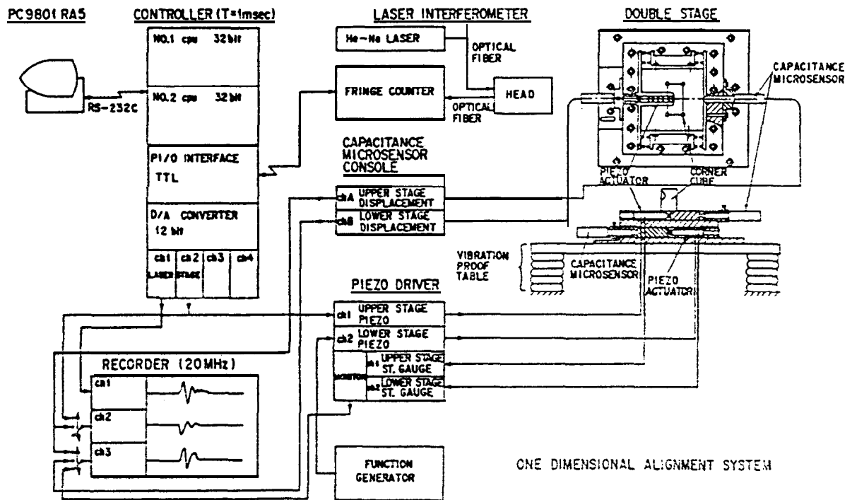
FIGURE 1 Block diagram of the test facility.
