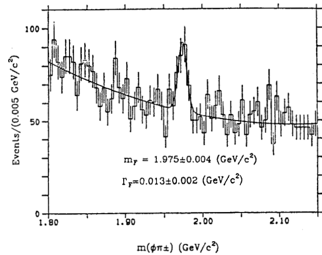
Figure 13. The \phi\pi mass spectrum from the HRS collaboration. The peak at 1975 MeV/c 2 is interpreted as the F seen by CLEO.
