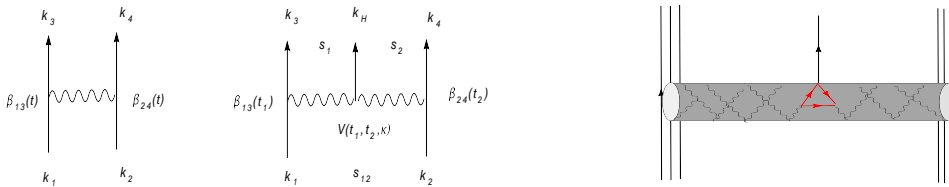
Figure 1: (a) Kinematics for single-Regge limit for 2-to-2 amplitudes, (b) Double-Regge kinematics for 2-to-3 amplitudes. (c) Cylinder Diagram for large N_c Higgs Production.
