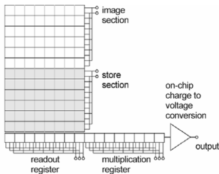
Figure1: EMCCD Schematic
